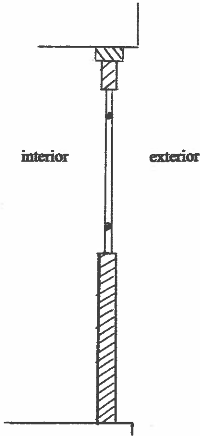
FRONT DOOR vertical section double glazed timber painted white
