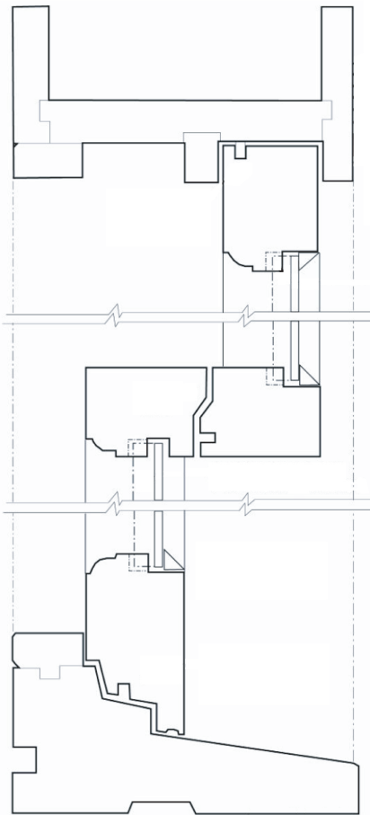
SECTION THROUGH WINDOW
