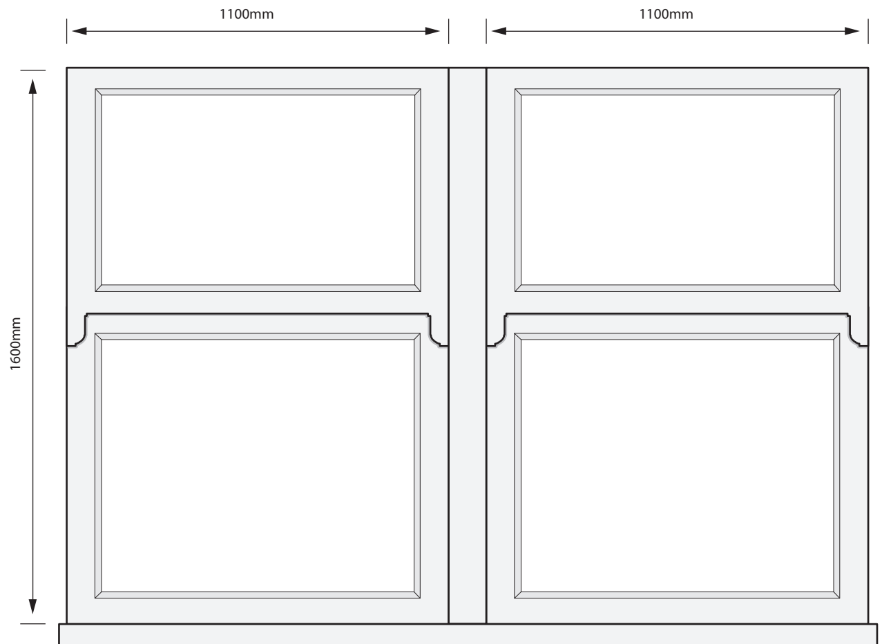
ELEVATION DRAWING
