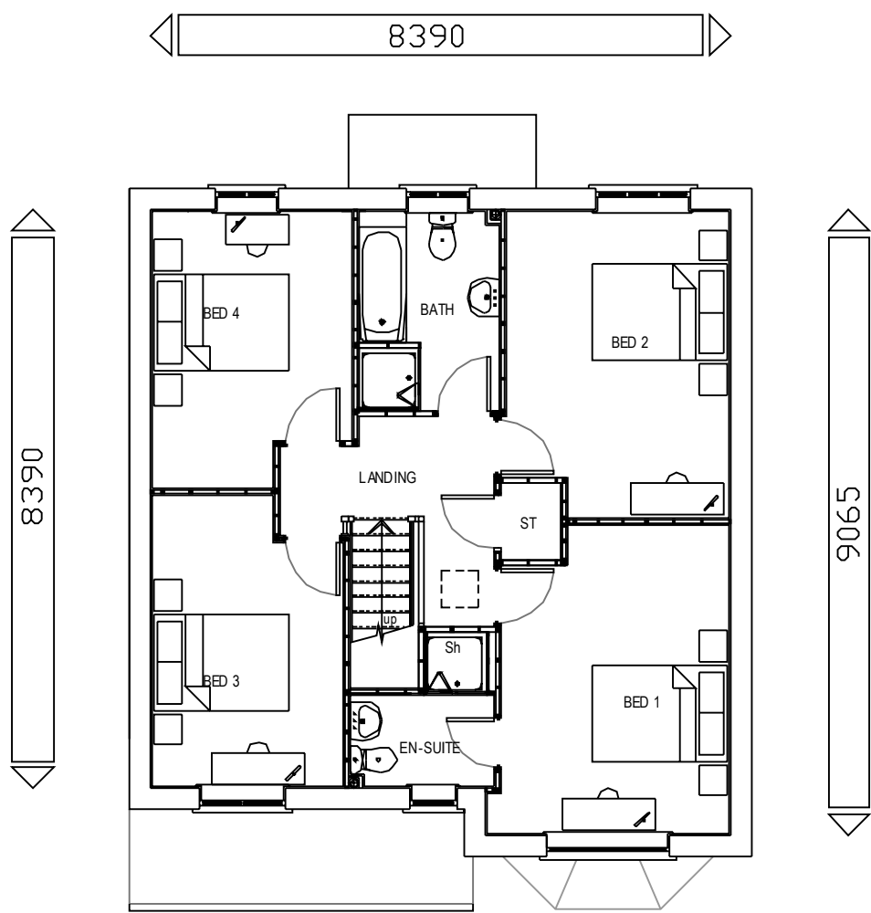
FIRST FLOOR
