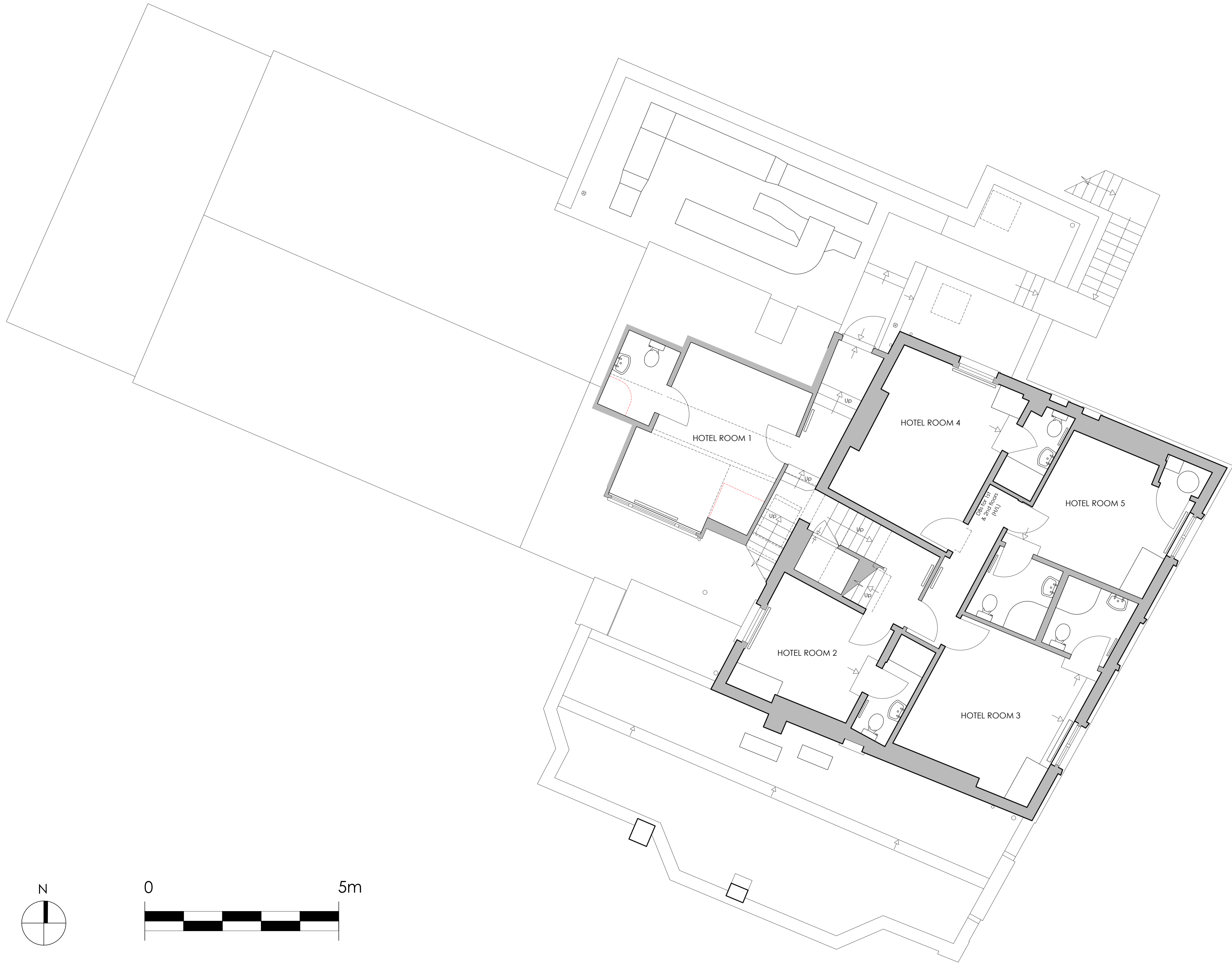
EXISTING FIRST FLOOR PLAN Scale 1:50
