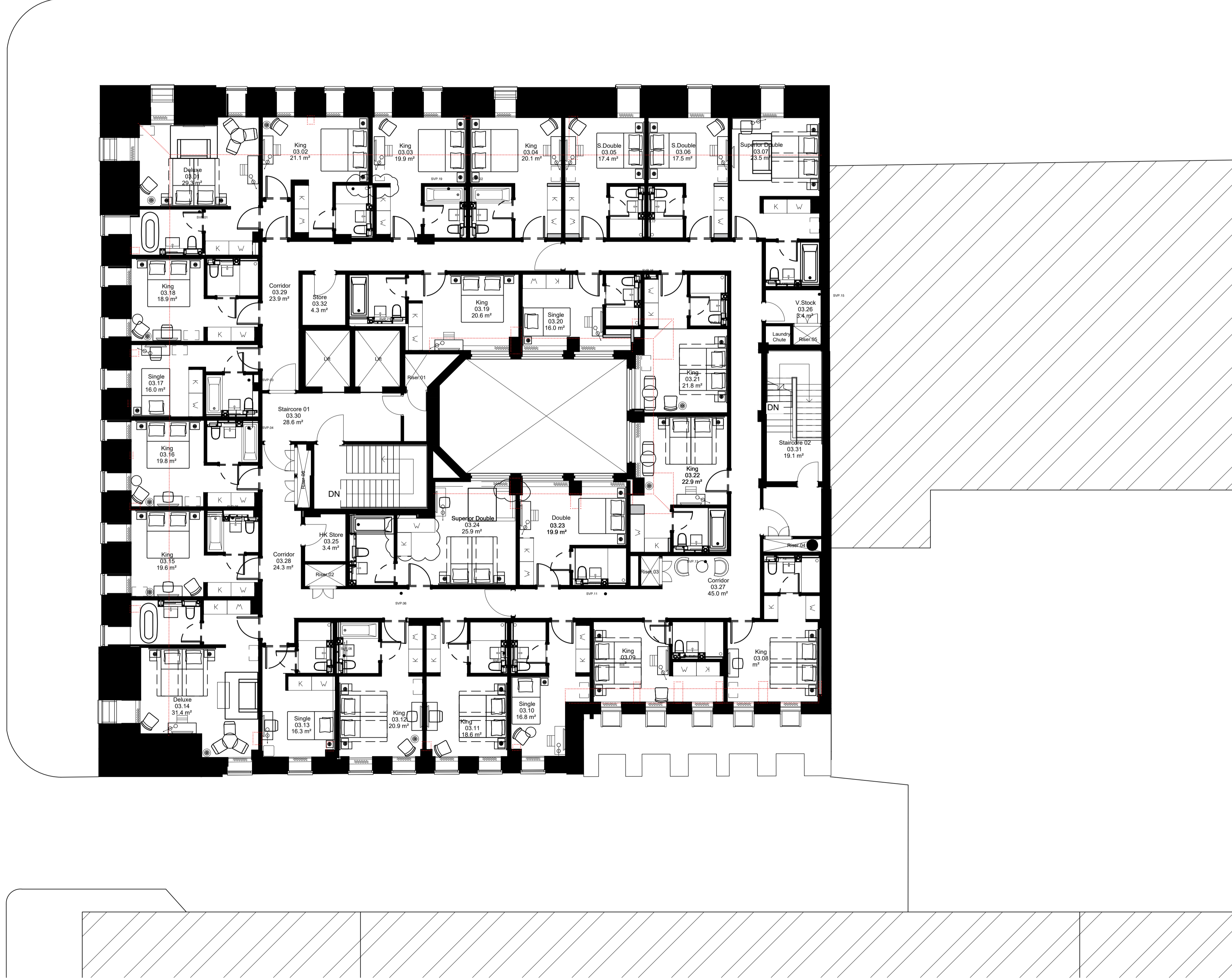
1 Wellington House - Existing Third Floor Plan 1 : 100
