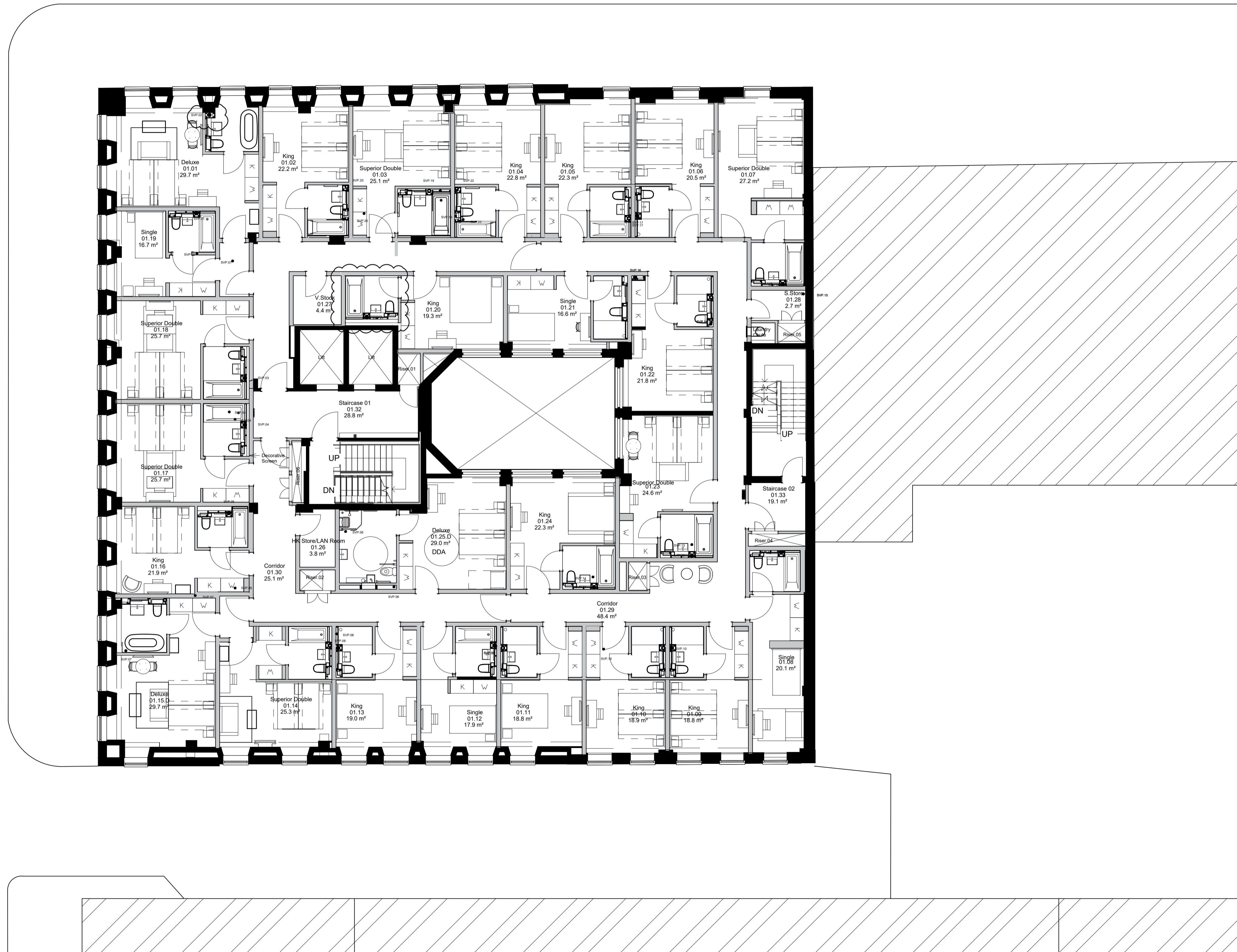
1 Wellington House - Existing First Floor Plan 1 : 100 0m 2m 4m 6m 8m
