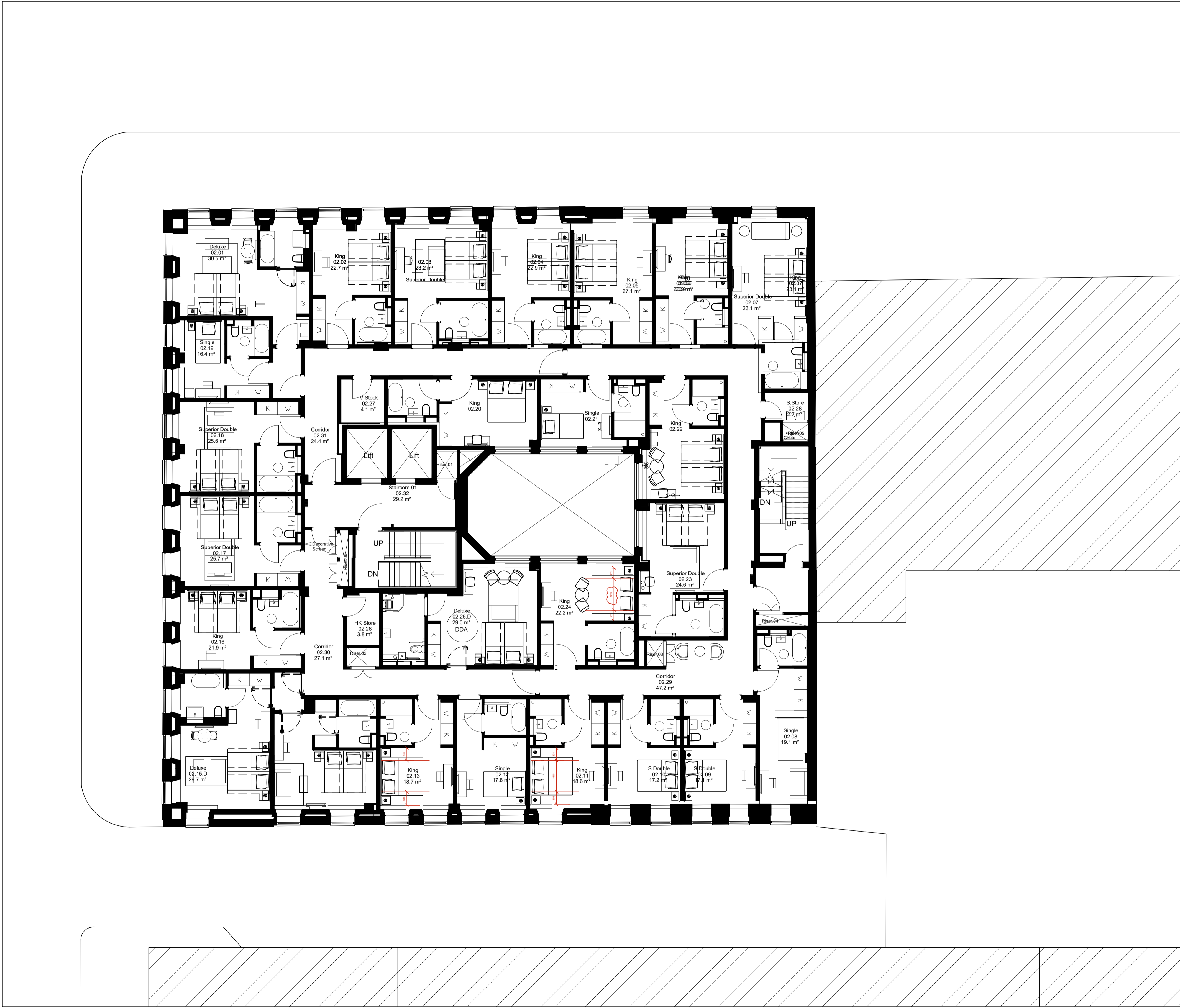
1 Wellington House - Existing Second Floor Plan 1:100
