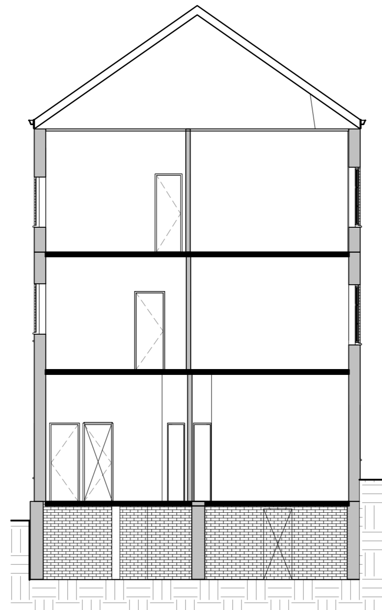
2 Section Proposed 1 : 100
