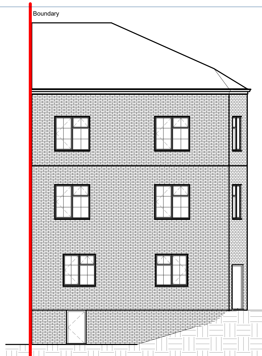
2 01. Front Elevation Proposed 1 : 100
