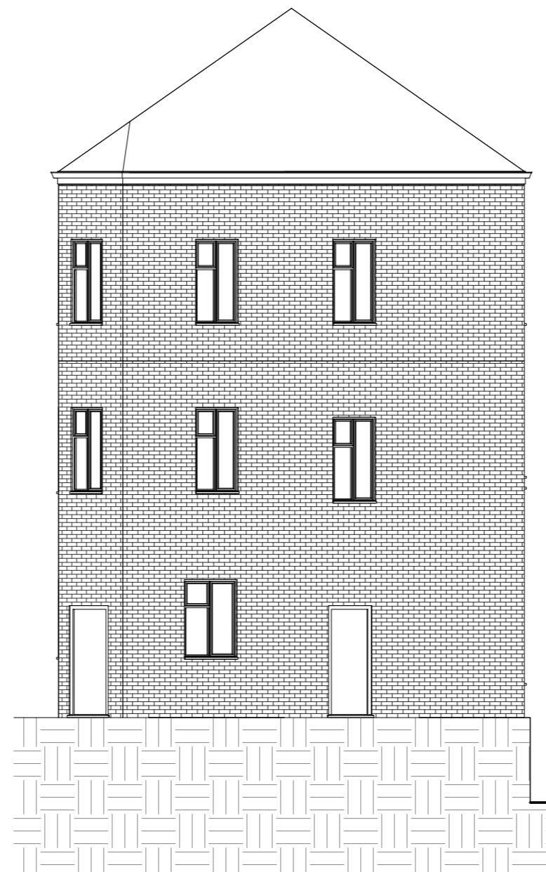
2 03. Right Elevation Proposed 1 : 100
