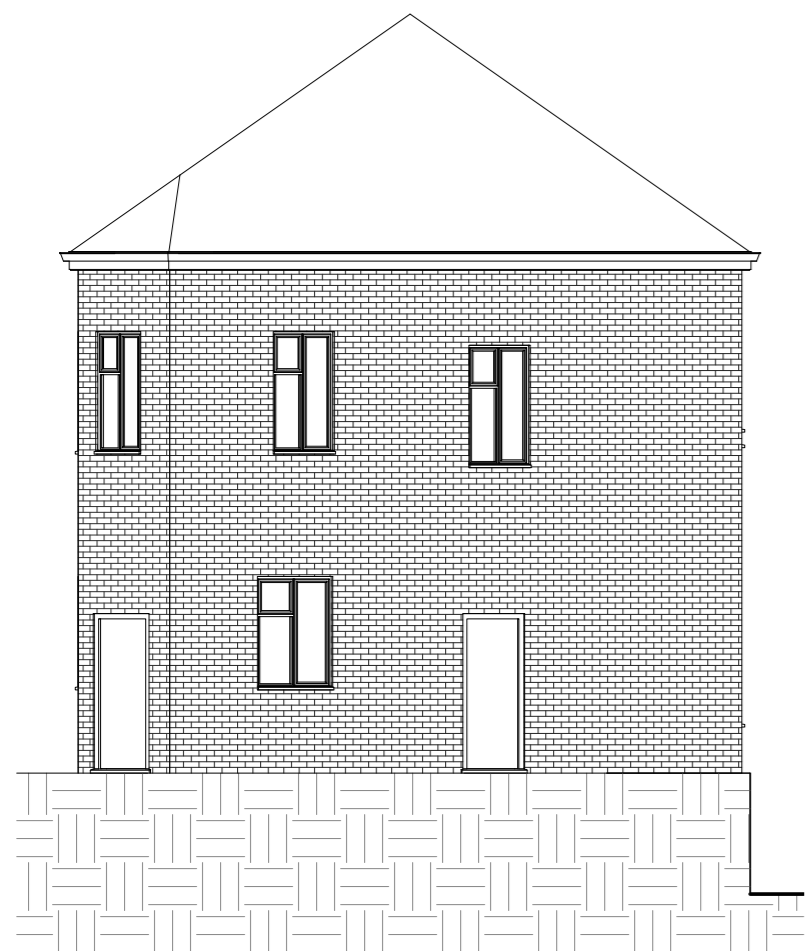
1 03. Right Elevation Existing 1 : 100
