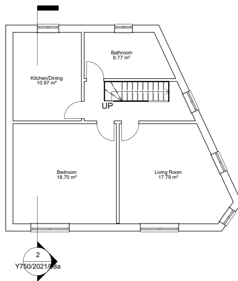
4 03. SF Proposed 1 : 100
