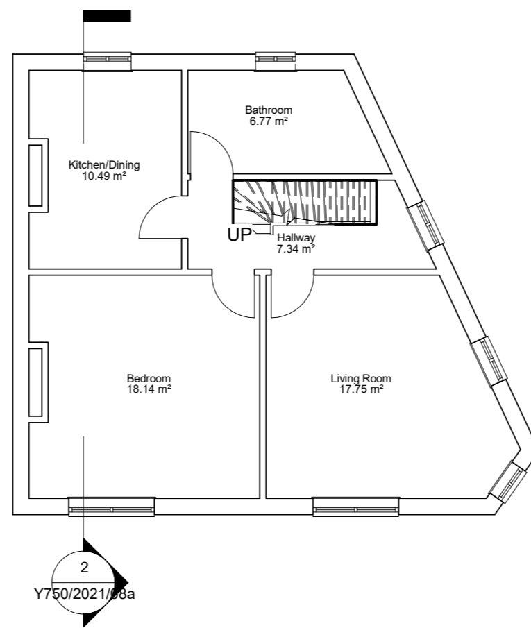
2 02. FF Proposed 1 : 100
