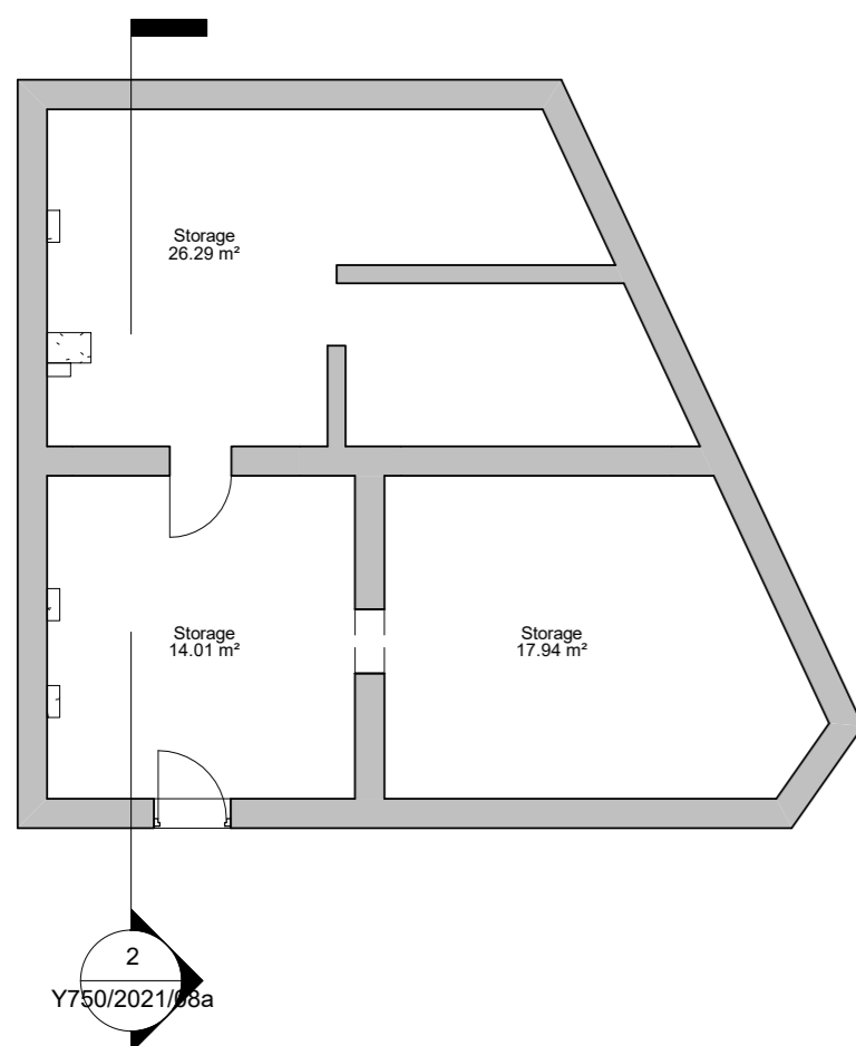
2 00. Basement Proposed 1 : 100
