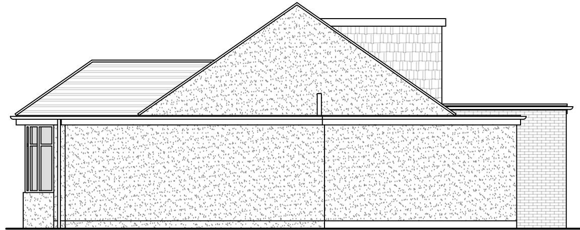
PROPOSED SIDE (South East) ELEVATION
