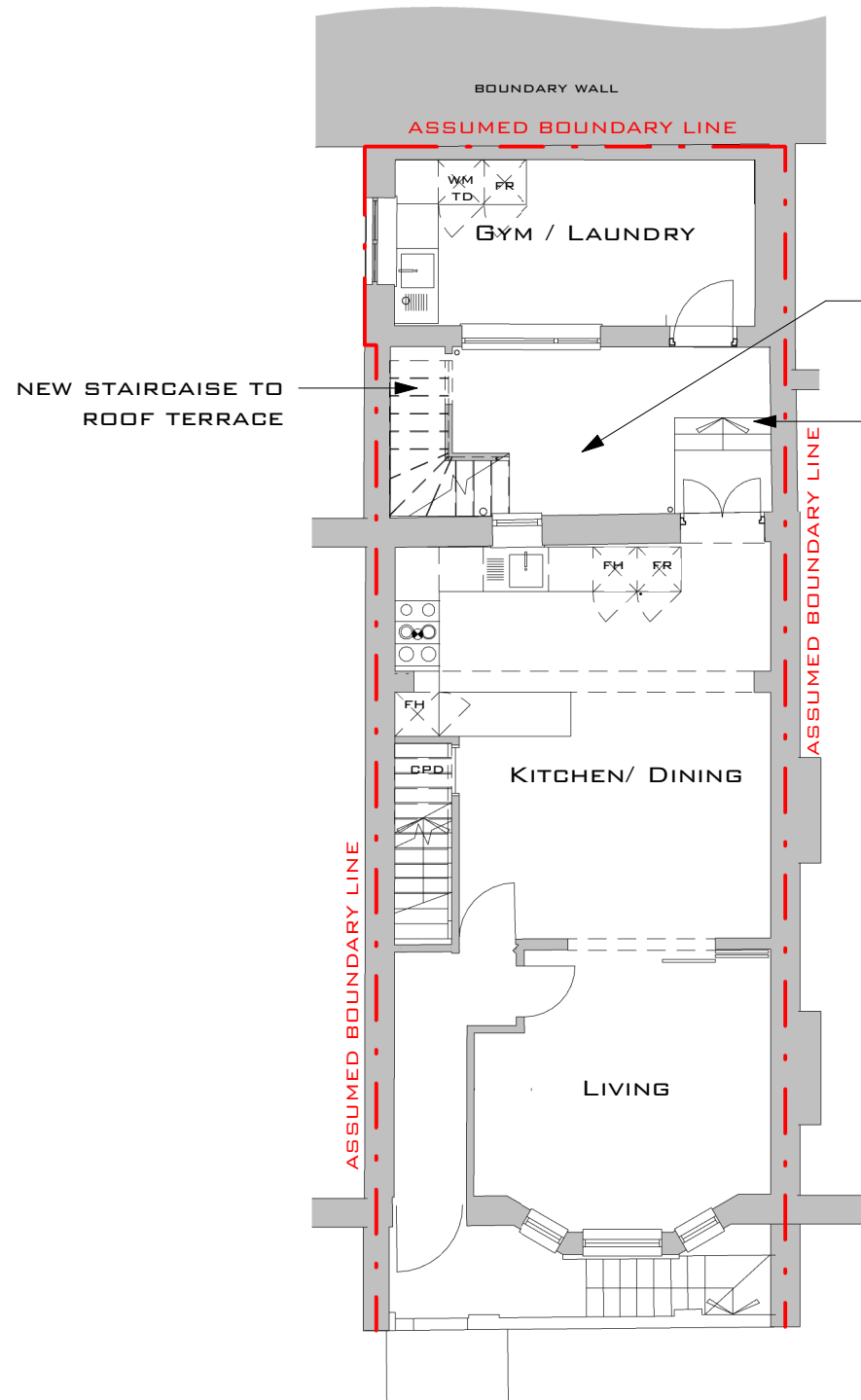
PROPOSED BASEMENT PLAN
