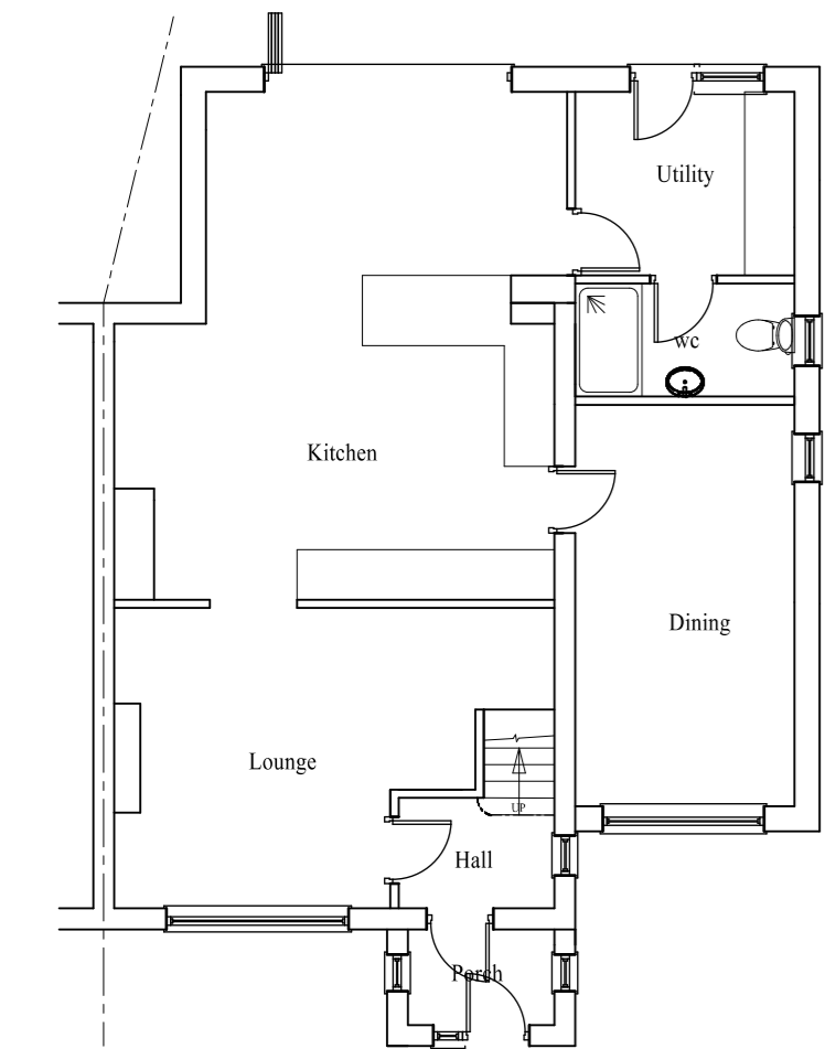
GROUND FLOOR (EXISTING)
