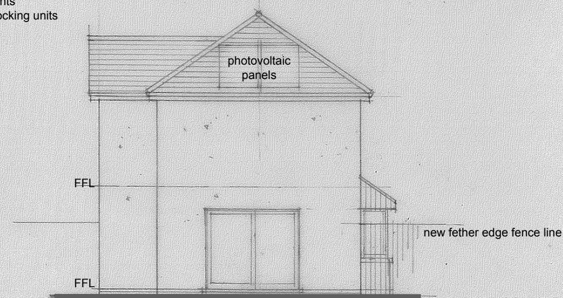
SIDE ELEVATION
