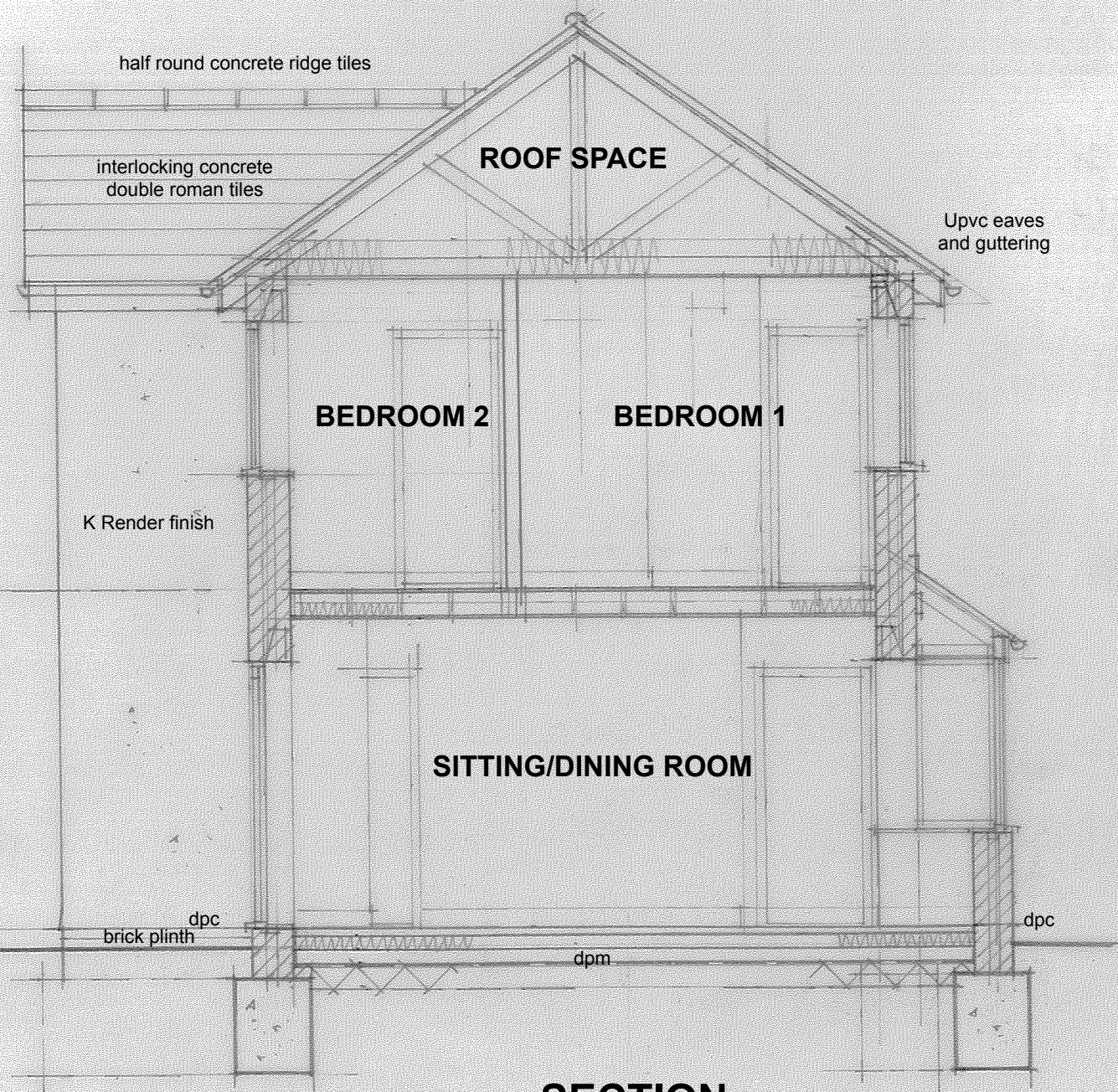
SECTION SCALE 1/50
