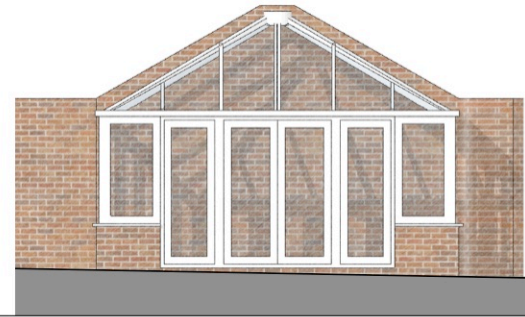
Existing Conservatory Elevation 1
