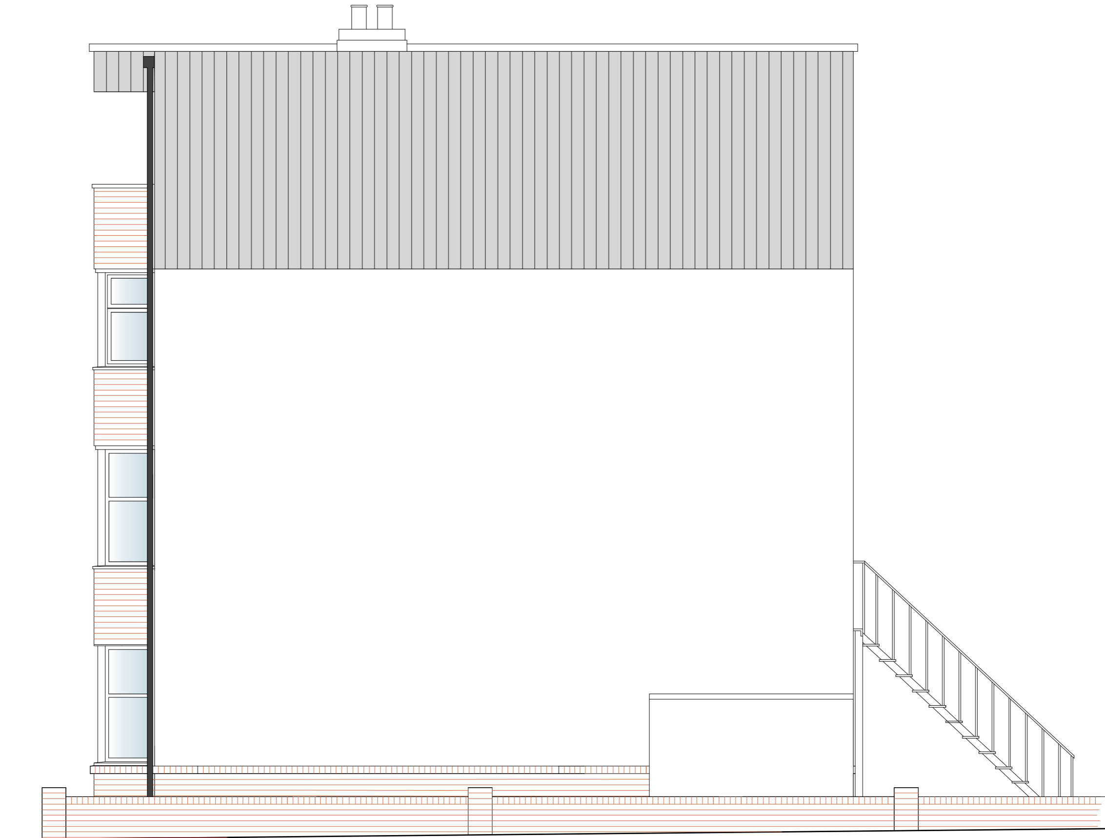
Side Elevation - East.
