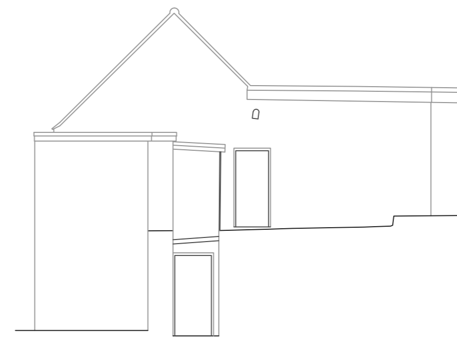
South elevation
