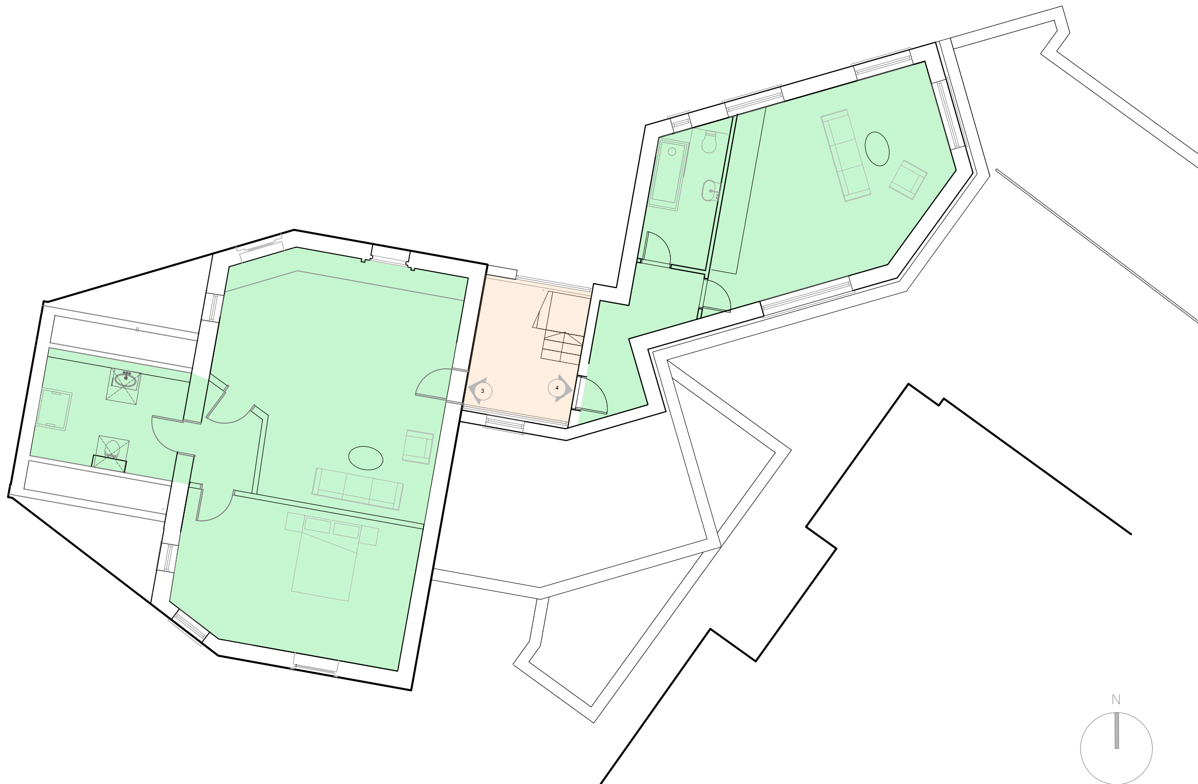
Second floor plan 1:100
