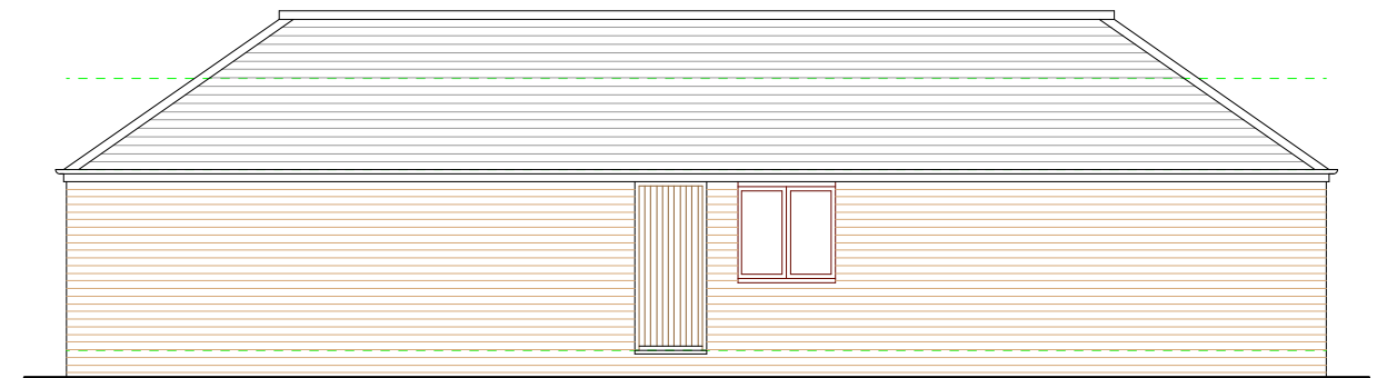
FRONT ELEVATION
