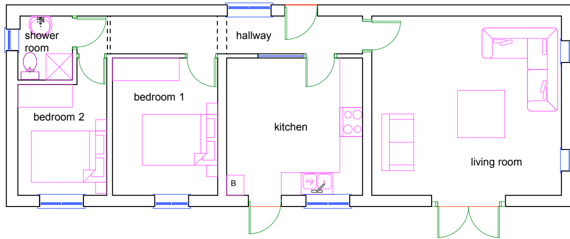
FLOOR PLAN
