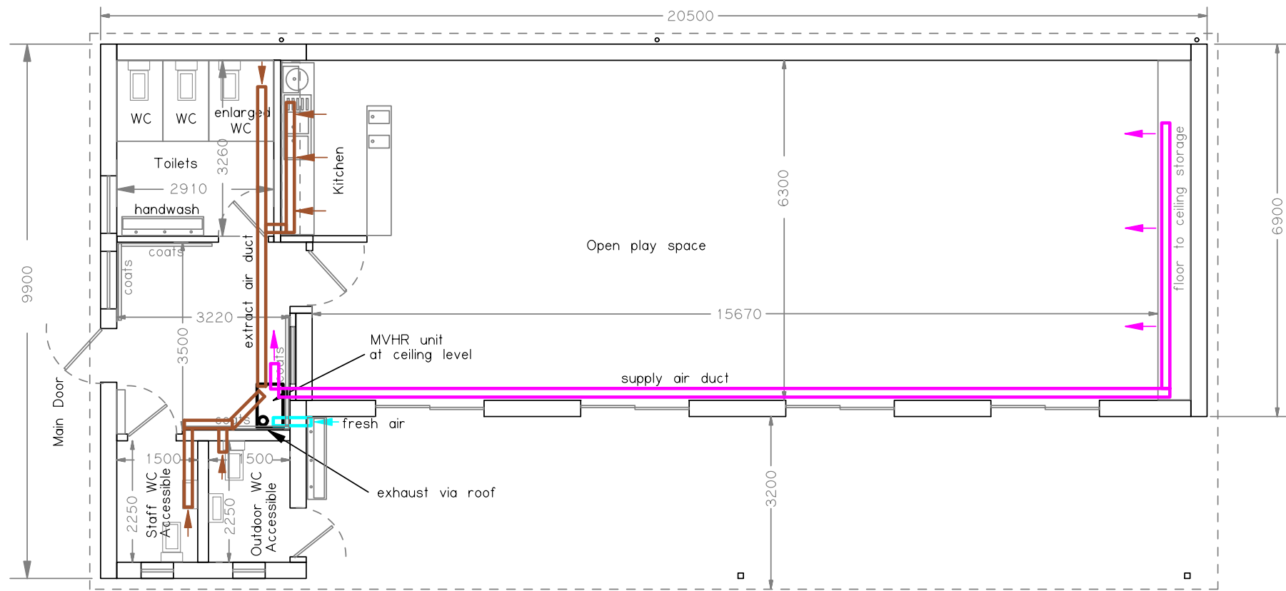
Ventilation Duct Route Plan
