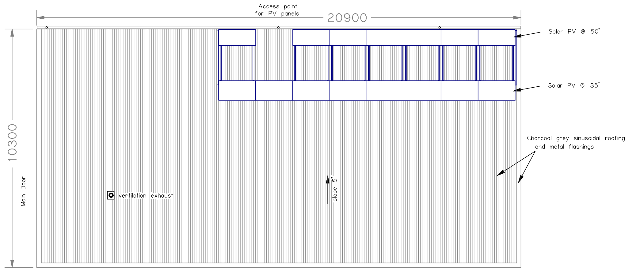
Roof Plan
