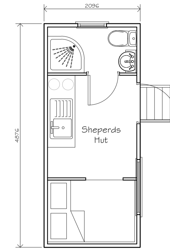
Floor Plan
