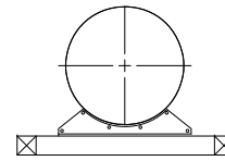
C102 MOUNT FEETS FIXING DETAILS TYPICAL
