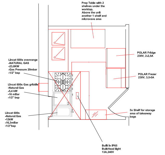
PROPOSED KITCHEN PLAN
