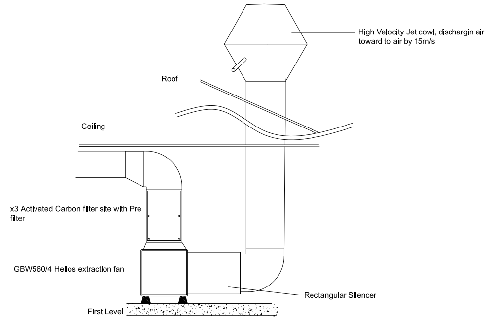
PROPOSED FAN 1-5 PLAN NOT SCALED
