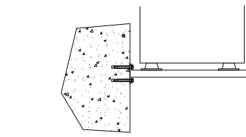
C100 STRUT WALL FIXING DETAILS TYPICAL
