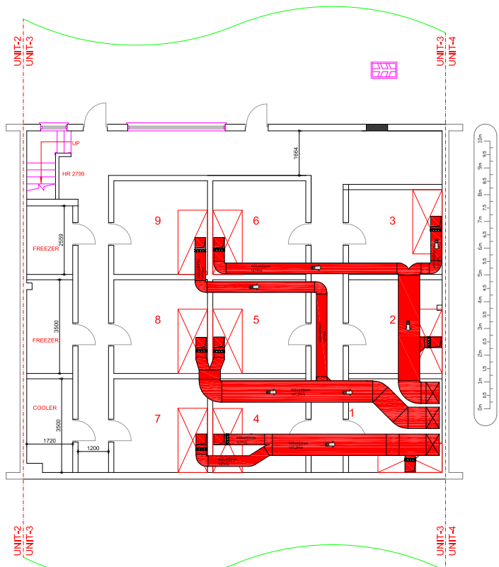
PROPOSED VENTILATION PLAN GROUND FLOOR
