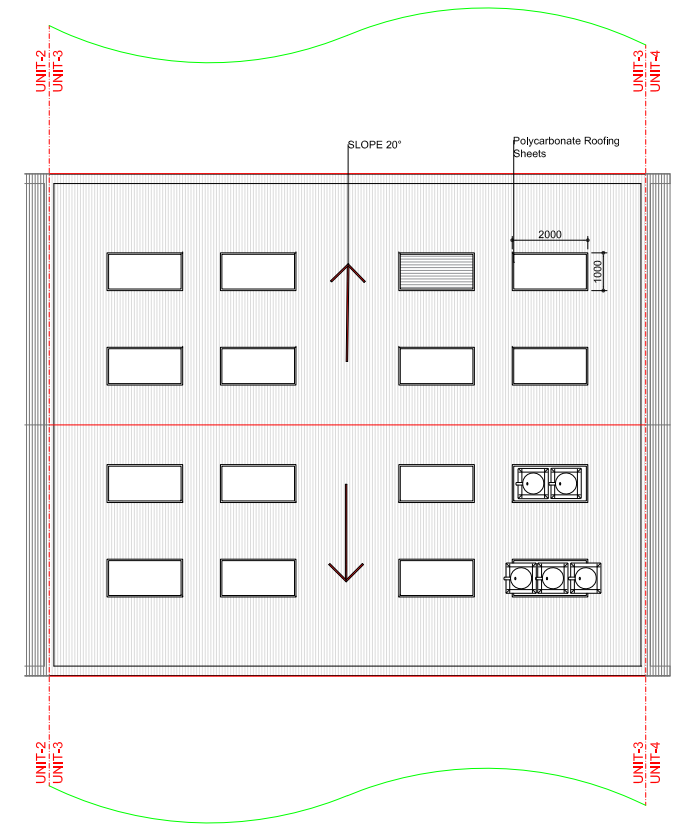
PROPOSED ROOF VIEW
