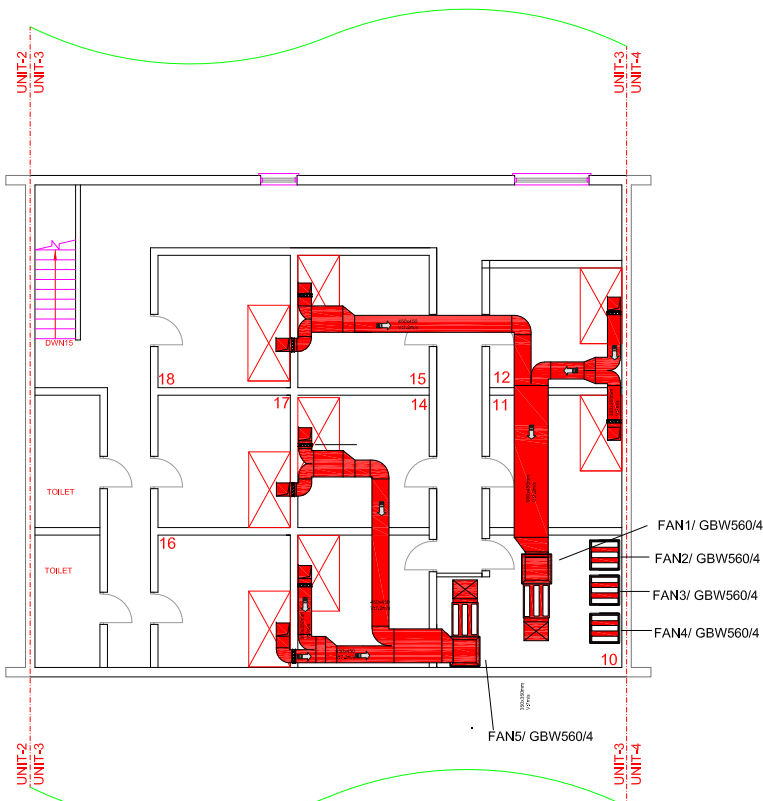
PROPOSED VENTILATION PLAN-FIRST FLOOR
