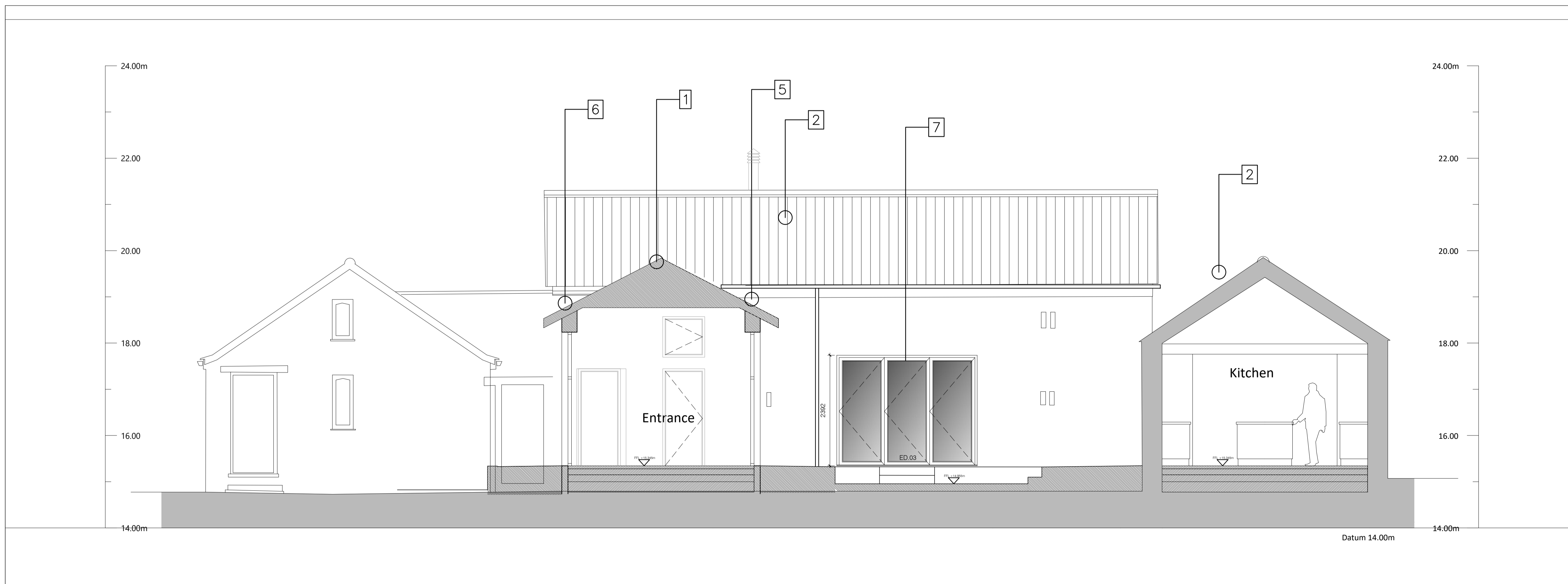
PROPOSED ELEVATION 02 - COURTYARD NORTH WEST
