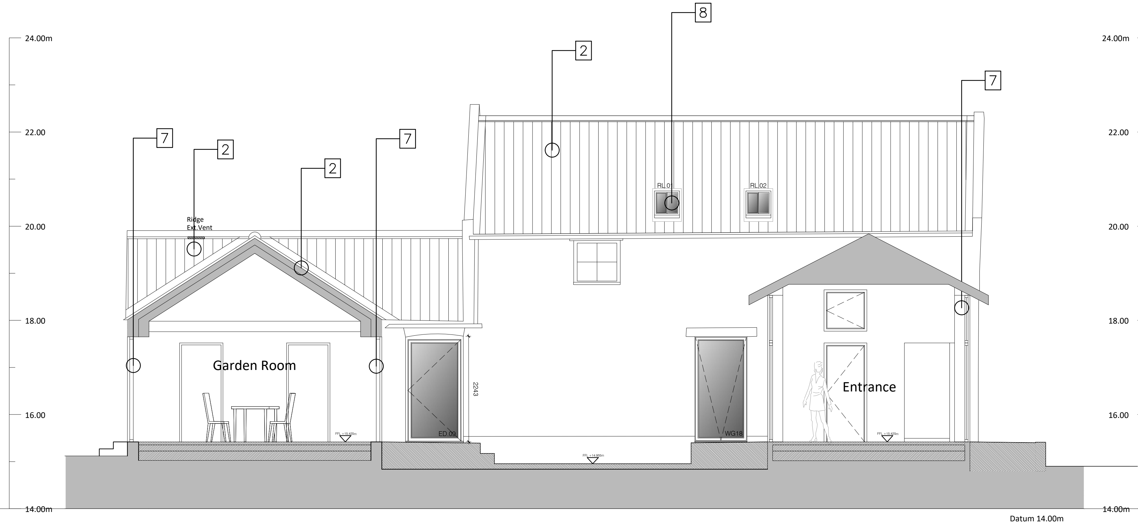
PROPOSED ELEVATION 04 - SOUTH EAST
