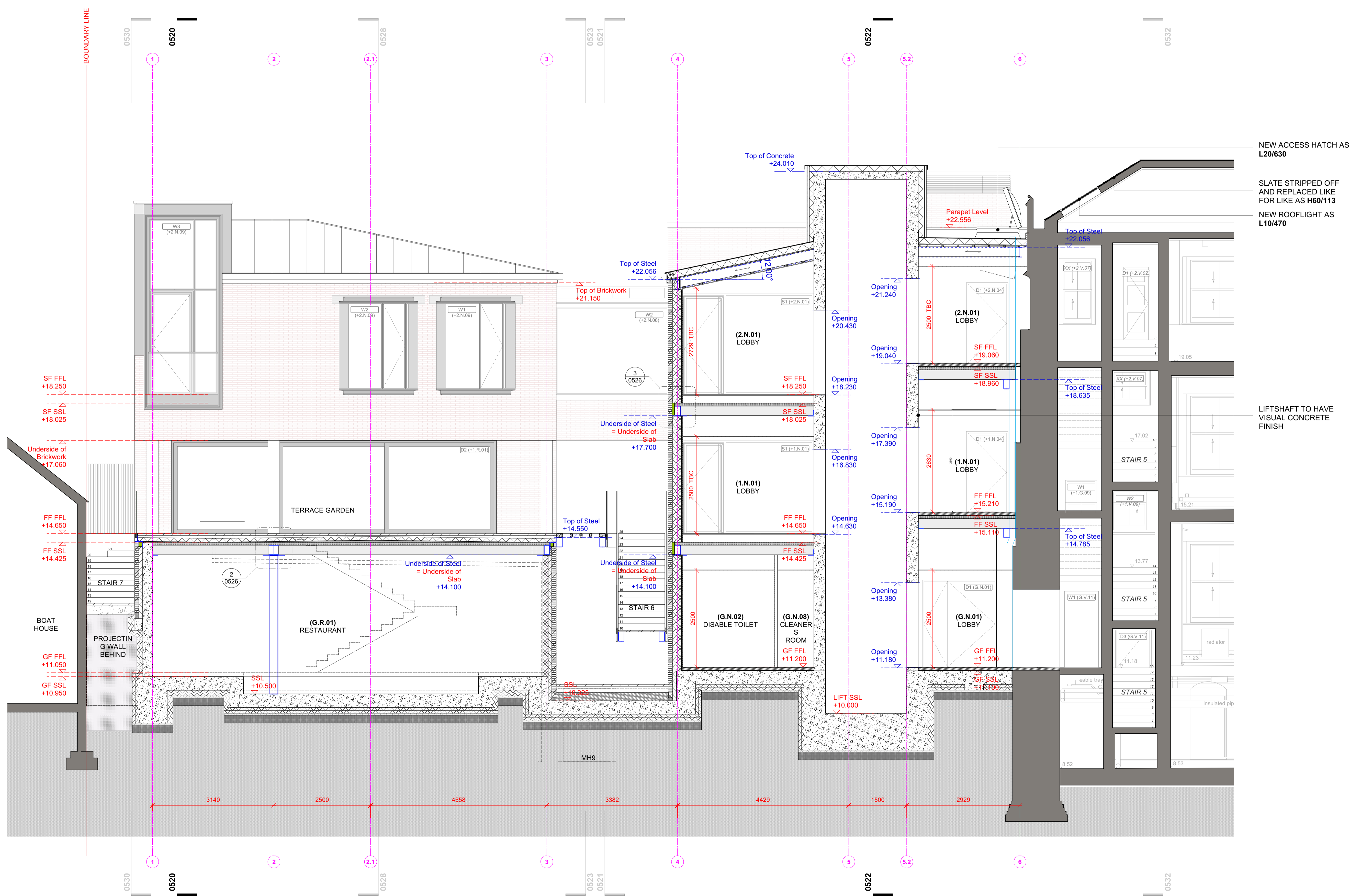
1 NORTH ANNEXE TRANSVERSE SECTION 3 1:50
