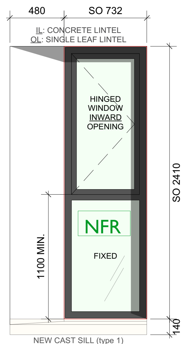
W6(+1.N.08) Window TYPE 12B SAS PRe with casement as L10/331
