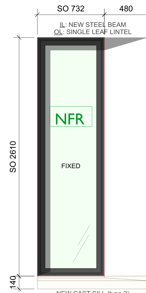
W2(+1.N.08) CW TYPE 9A SAS SF 52 Curtain Walling as H11/111
