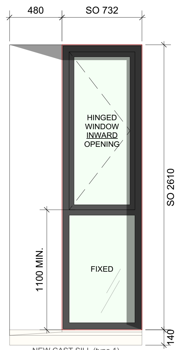
W6(+2.N.08) Window TYPE 12B SAS PRe with casement as
