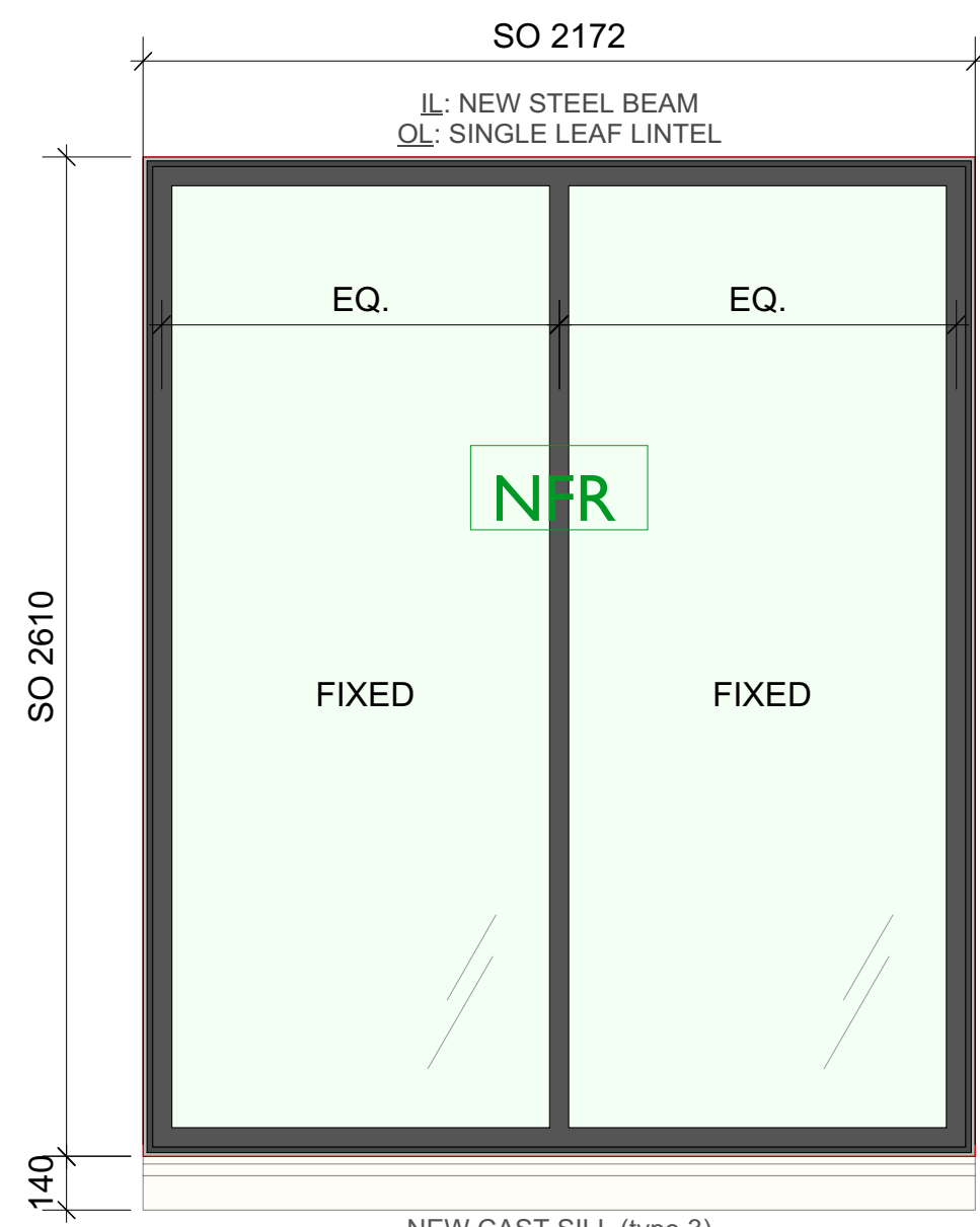
W1(+2.N.01) CW TYPE 9B - SAS SF 52 Curtain Walling - Multiple Fixed panes - as H11/111
