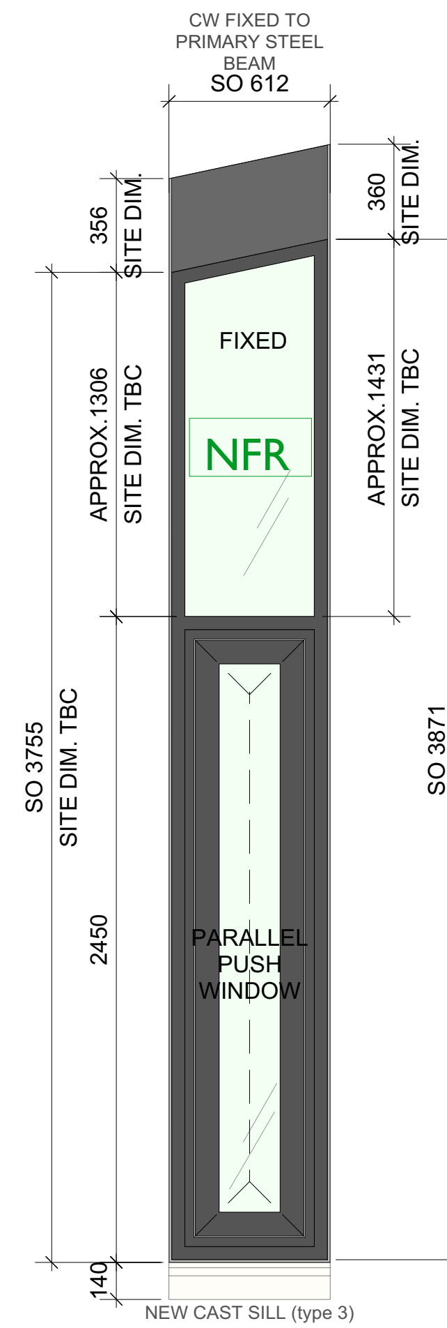
W4(+2.N.09) CW TYPE 9B SAS SF 52 Curtain Walling as H11/111 with PRe Parallel Push window inset at L10/331
