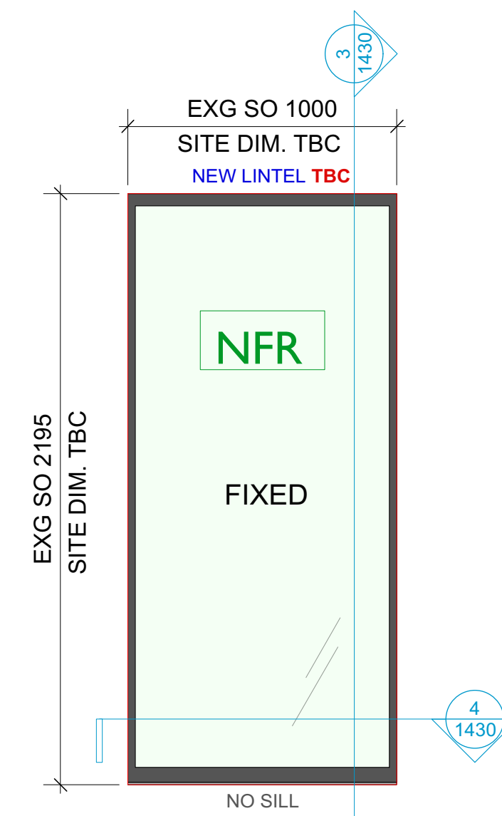
W3(G.V.02) Window TYPE 12A SAS PRe Fixed Window as L10/331
