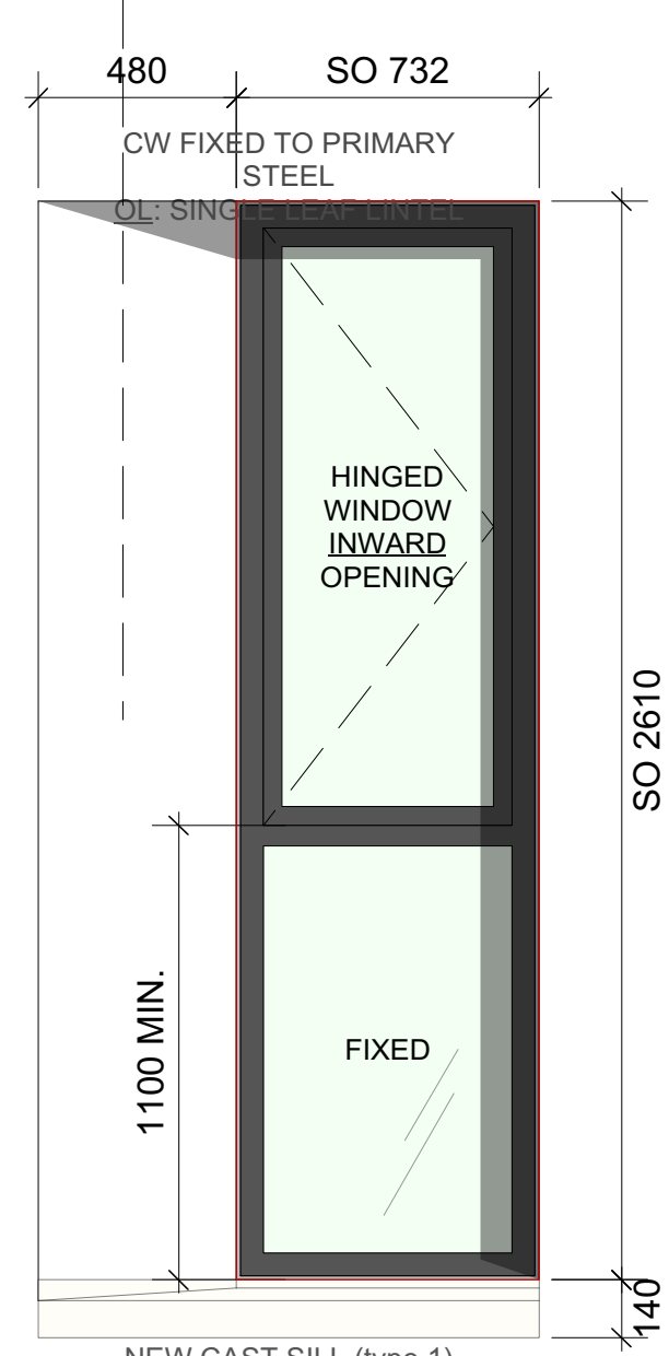
W5(+2.N.08) Window TYPE 12B SAS PRe with casement as
