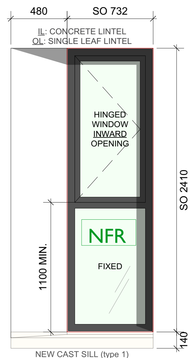
W5(+1.N.08) Window TYPE 12B SAS PRe with casement as L10/331
