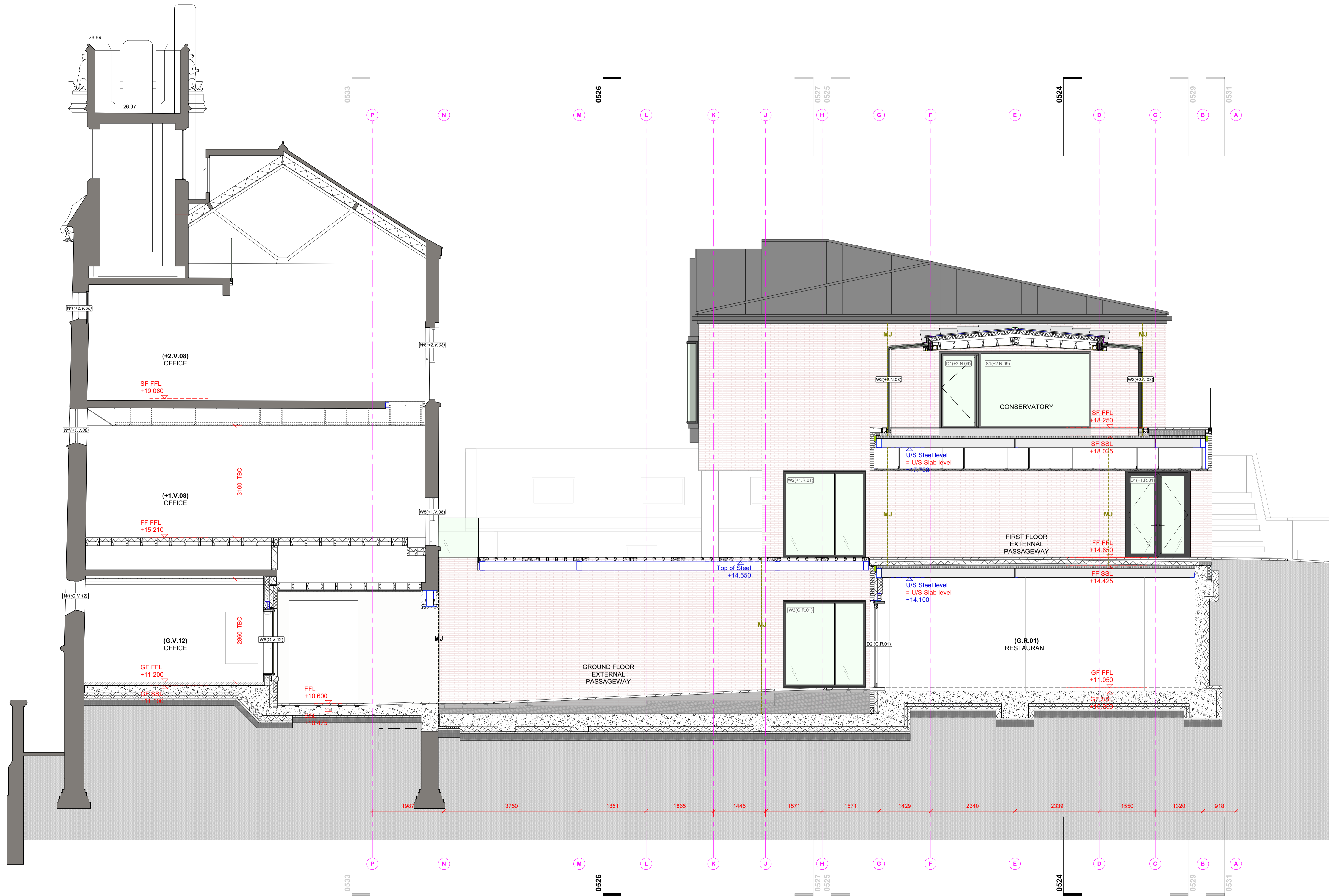
1 NORTH ANNEXE LONG SECTION 4 1:50
