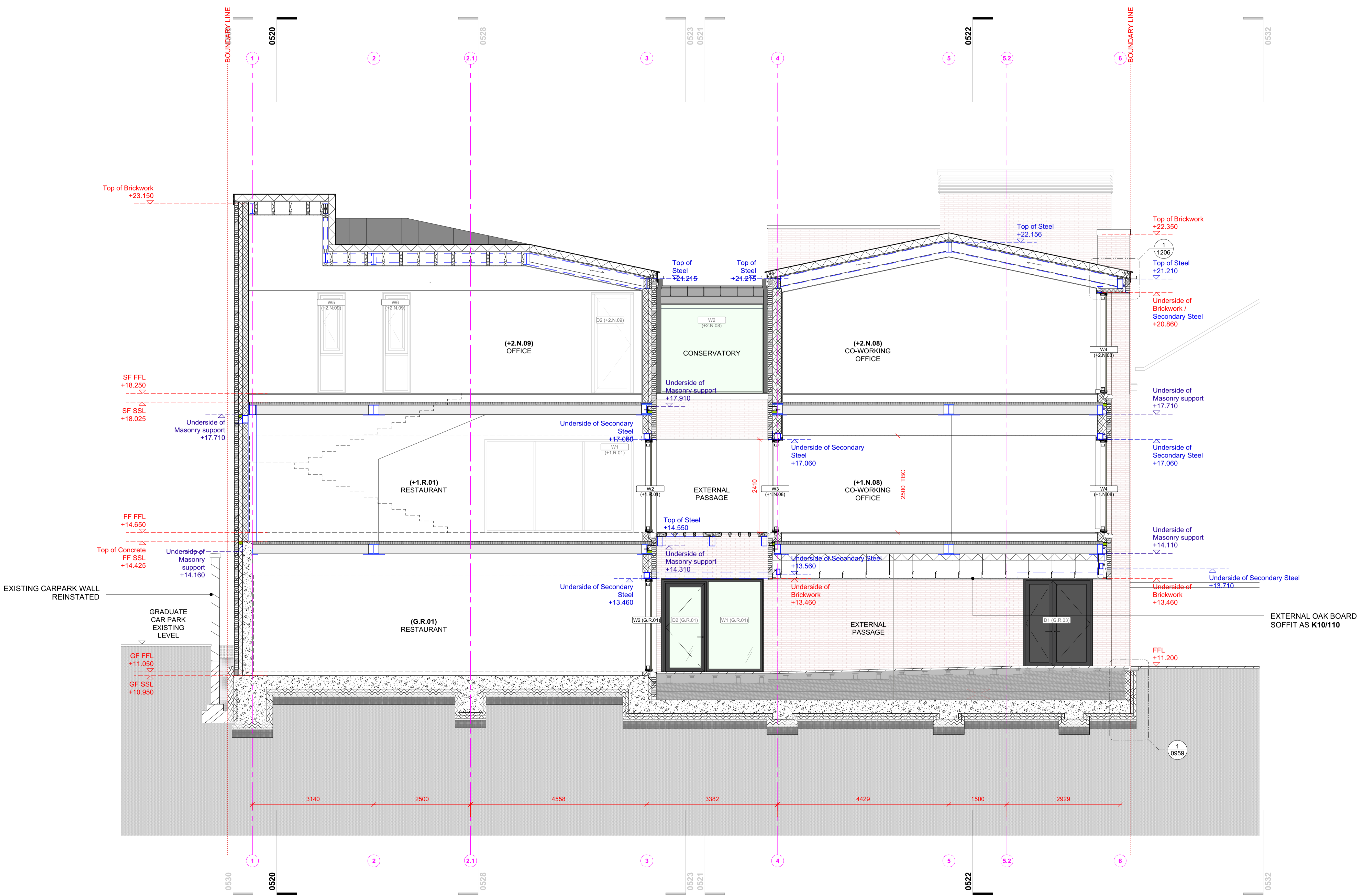
3 NORTH ANNEXE TRANSVERSE SECTION 2 1:50
