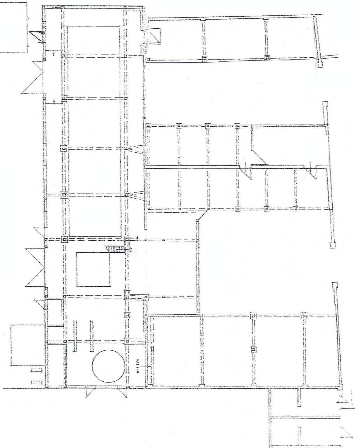
Southern Barn- Existing Plan 1:200 Scale
