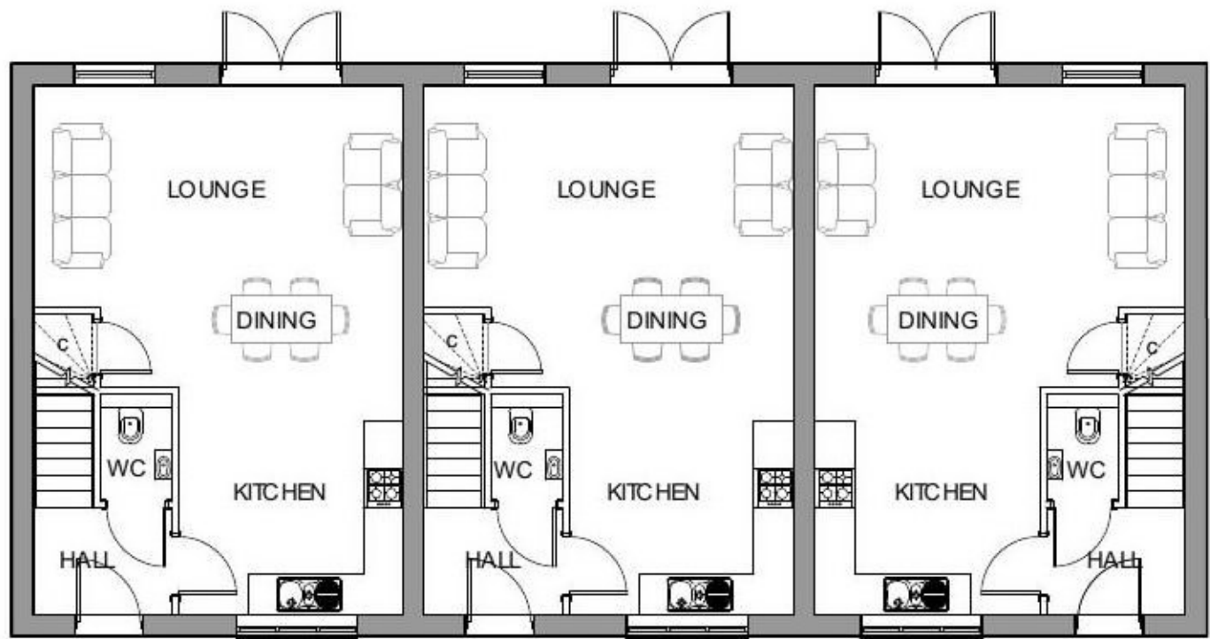
GROUND FLOOR PLAN - House Type 25 SCALE 1:100
