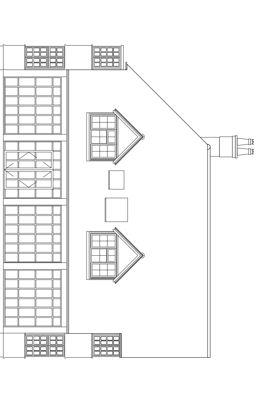
EXISTING WEST ELEVATION 1:100
