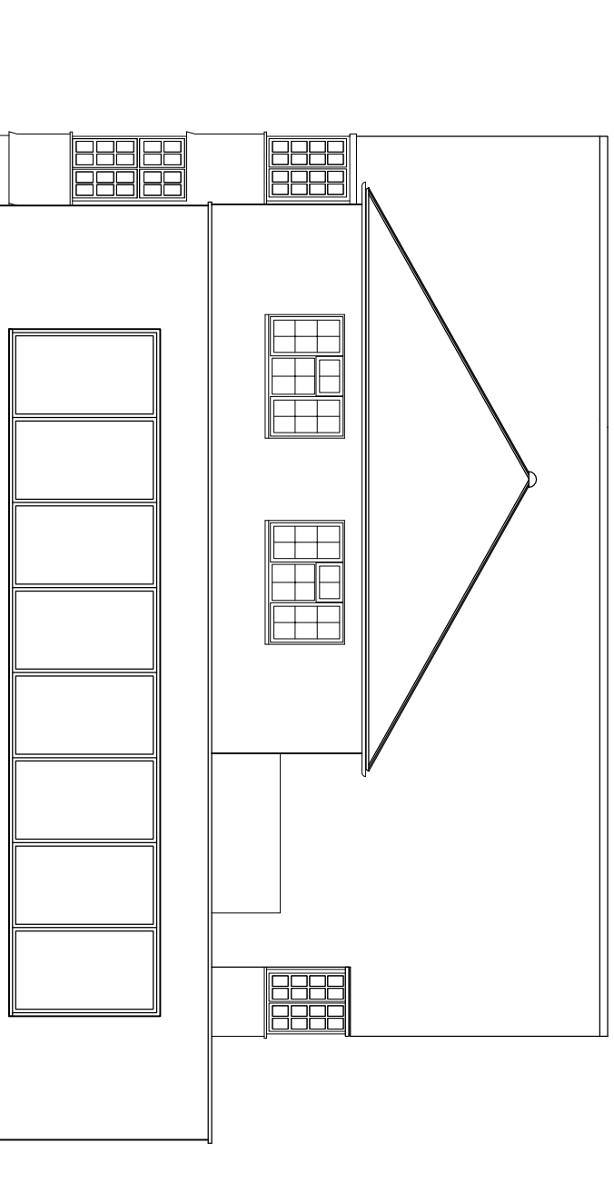
PROPOSED WEST ELEVATION 1:100
