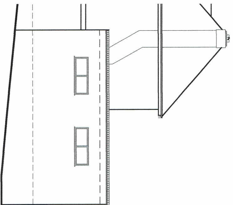
SIDE ELEVATION (PROPOSED)
