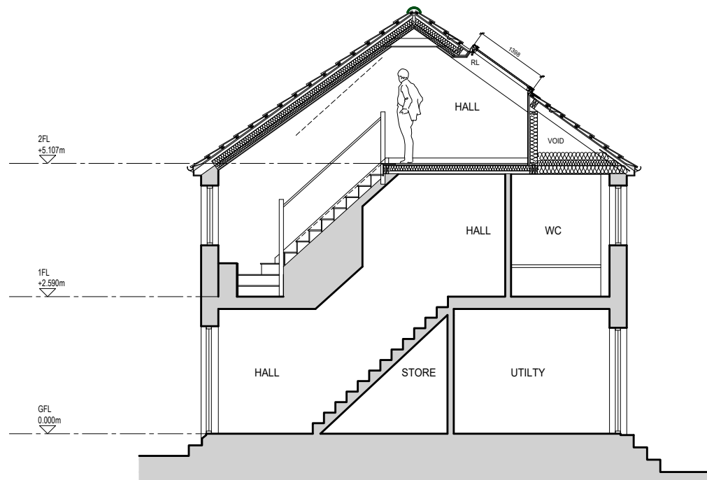
Section AA as Proposed
