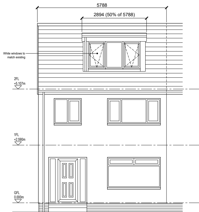
Front Elevation as Proposed
