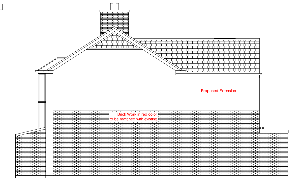
PROPOSED SIDE -B - ELEVATION
