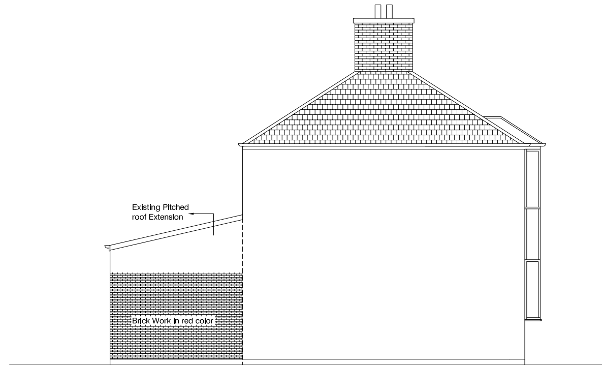
EXISTING SIDE -A - ELEVATION
