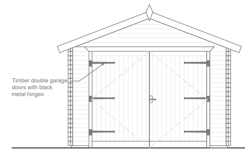
Proposed Front Elevation 1:50@A1
