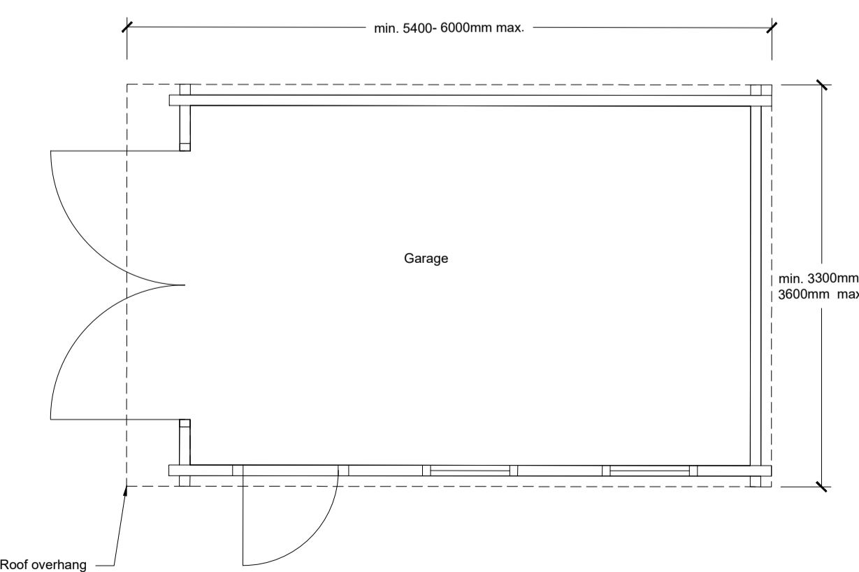
Proposed Garage Plan 1:50@A1
