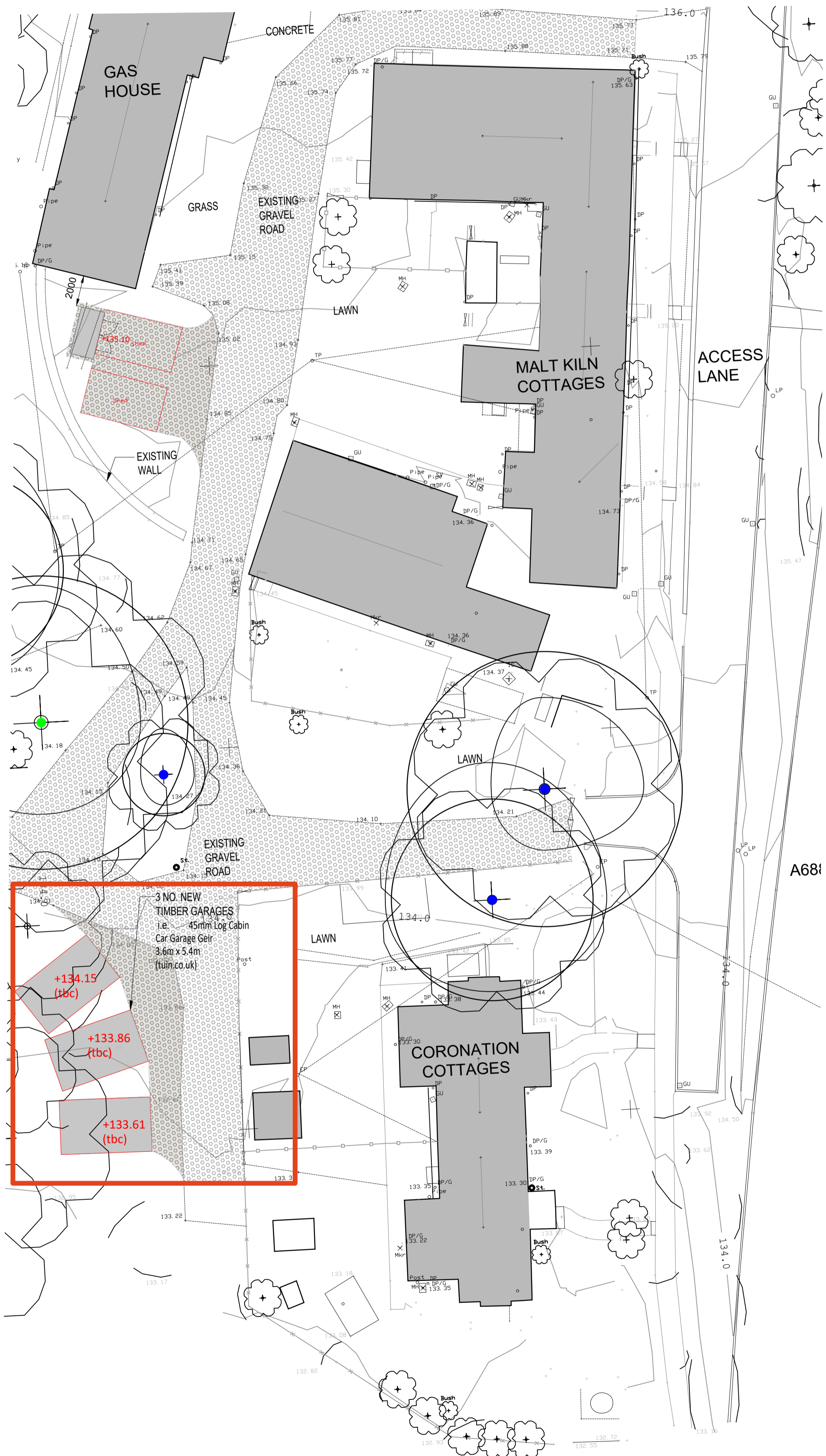
Proposed Garages Location Plan 1:200@A1
