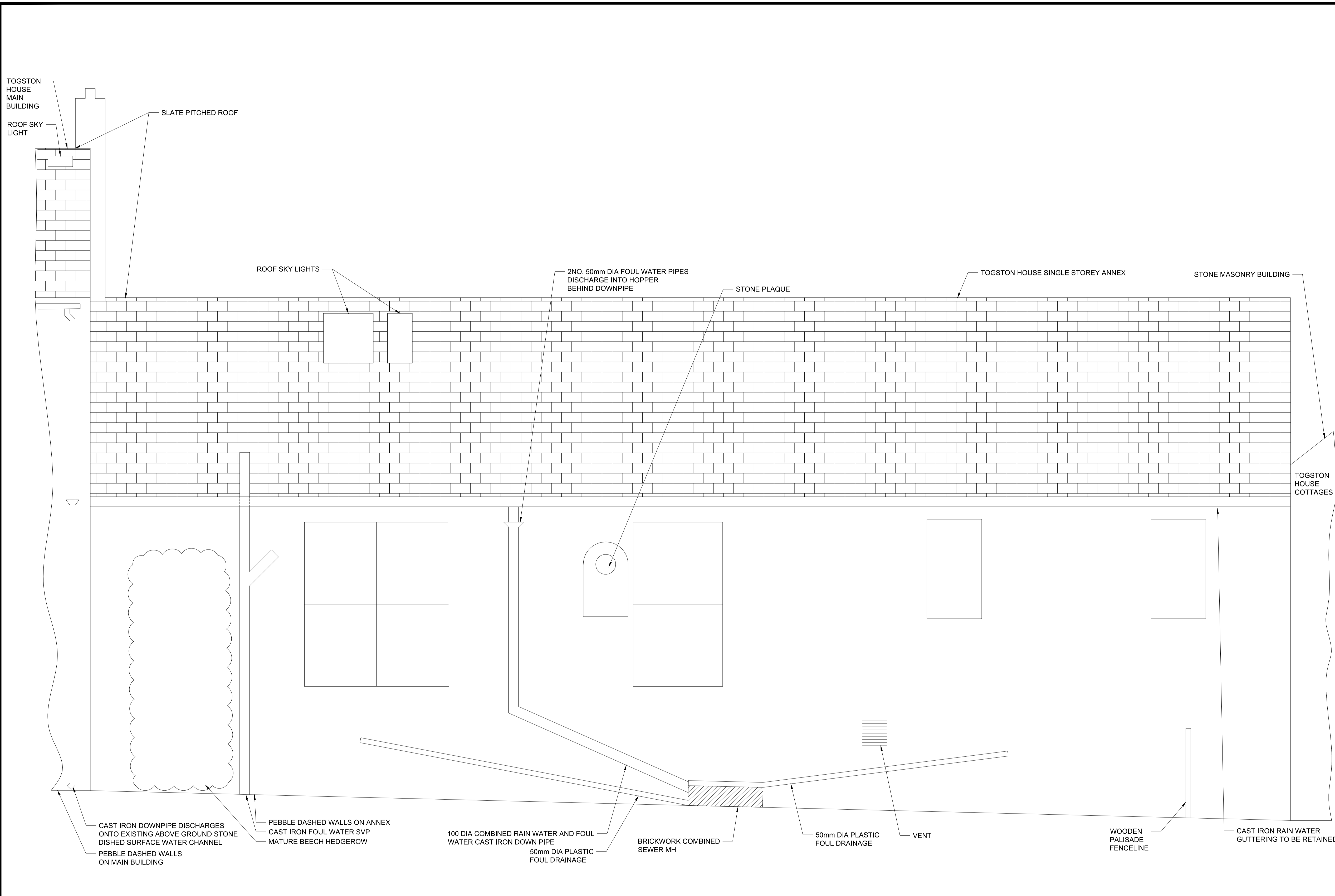
SOUTH ELEVATION SCALE 1:20
