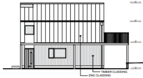
SIDE (NORTH) ELEVATION 1:100
