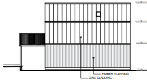
SIDE (SOUTH) ELEVATION 1:100
