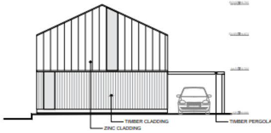
FRONT (EAST) ELEVATION 1:100
