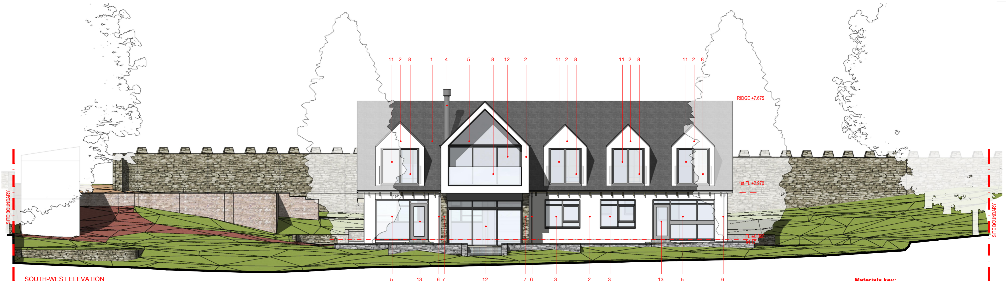
SOUTH-WEST ELEVATION
