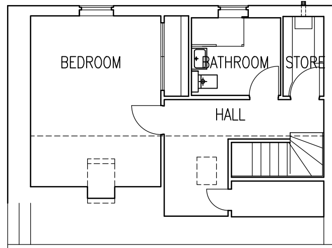
ATTIC PLAN
