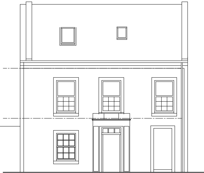
ELEVATION TO BATH STREET (S.E.)
