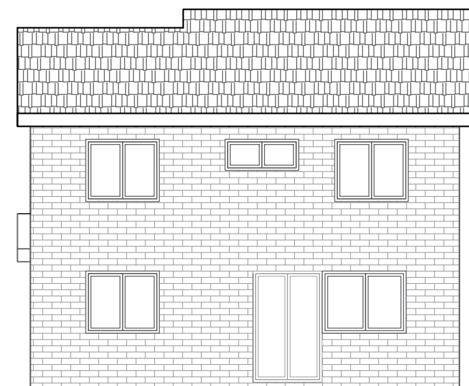
Proposed Rear Elevation same as Existing
