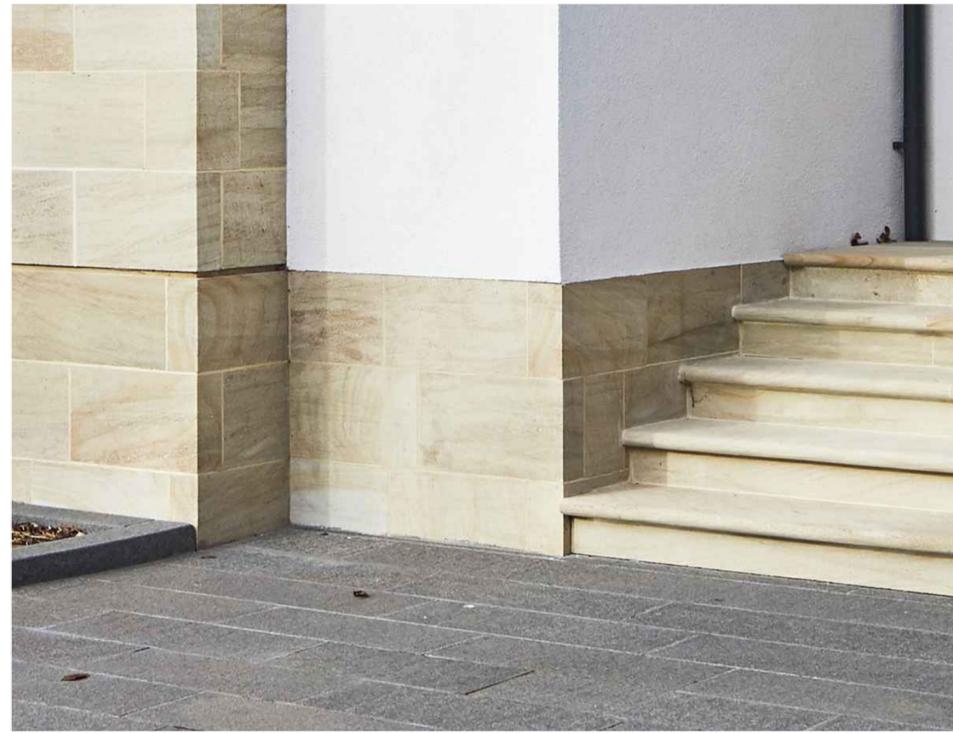
D.2 - Stone Plinth / Render Detail
