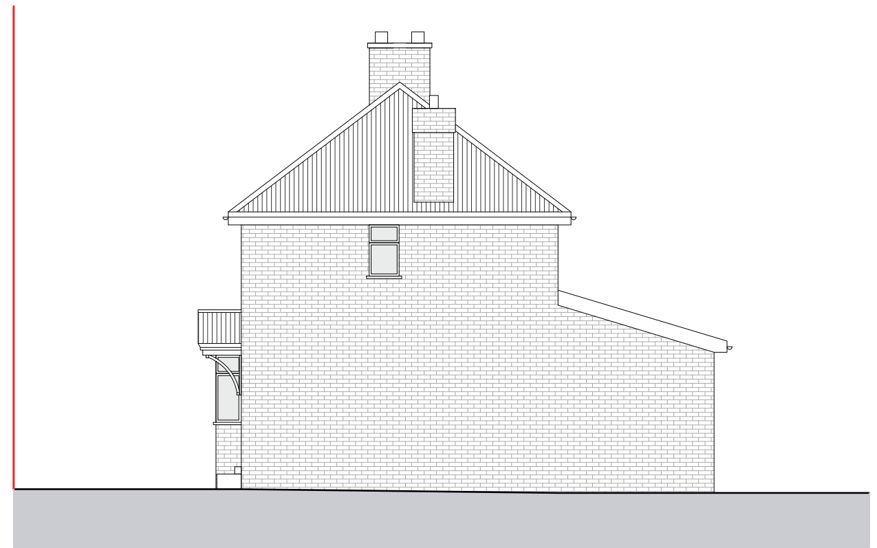
02.SIDE ELEVATION
