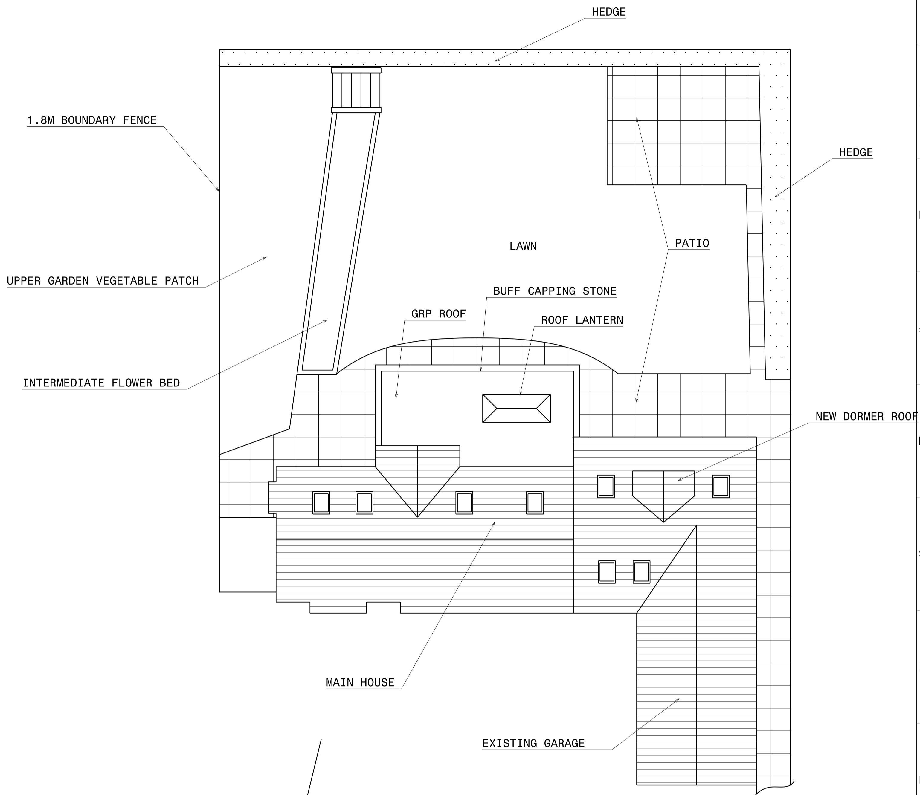
PROPOSED PLOT VIEW SCALE: 1:100
