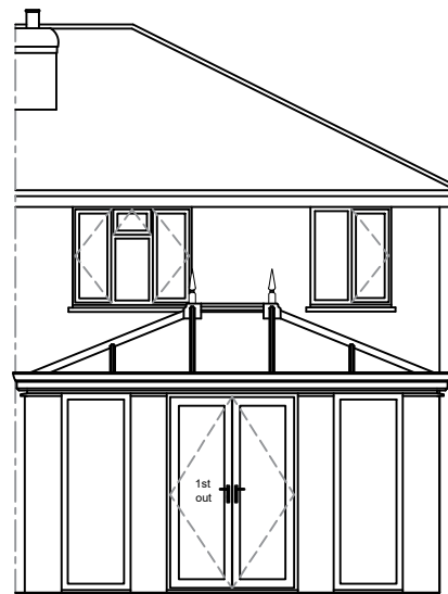
REAR ELEVATION
